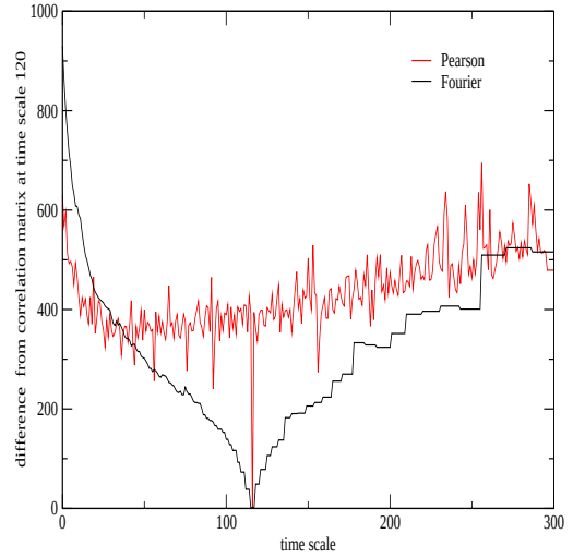
Figure 11: Differences from 2 hours time scale \sum_{i,j} |c_{ij}(t) - c_{ij}(120)| : left - MST, right - correlation matrices, Fourier - black, Pearson - red
