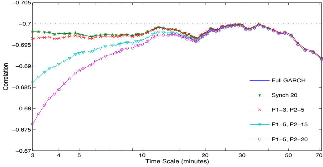
Figure 3: Simulated bivariate GARCH(1,1) - Fourier method
