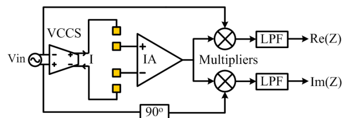
Fig. 1. Single frequency synchronous detection (also known as synchronous-, quadrature- or phase sensitive- demodulation and lock-in).
