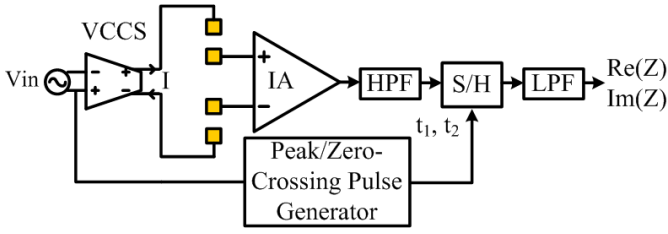
Fig. 2. Single frequency synchronous sampling.
