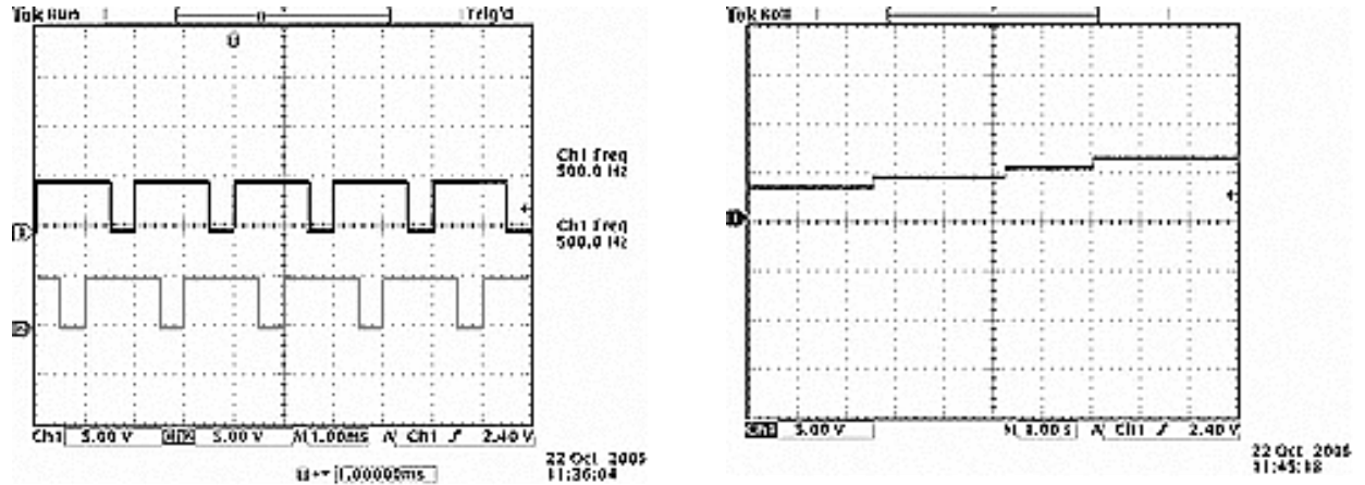
Figure 3. (a) Multiplexing signals from VI, used to control the multiplexing of the two emitters, and (b) Intensity signal from VI, which allows the intensity of the emitters to be varied. Each volt corresponds to 10mA of a drive current. The signal can be changed at anytime during use.
