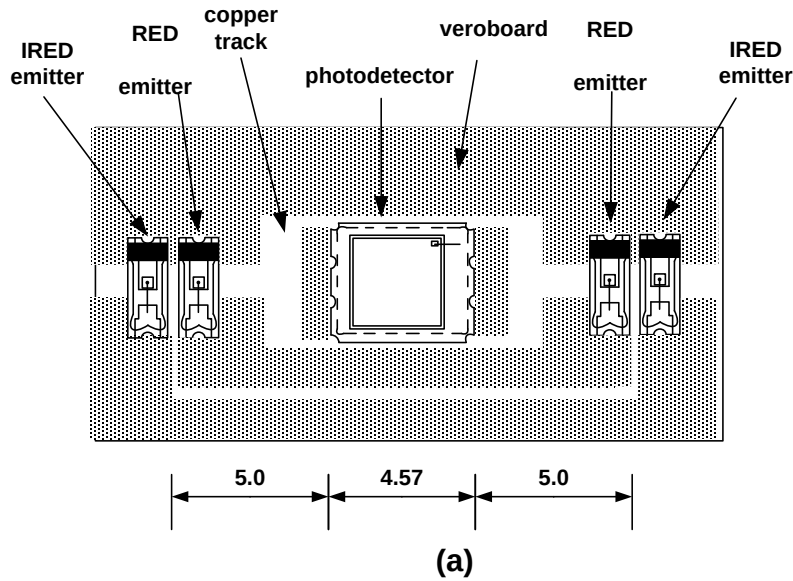
Figure 1: (a) Top view of the custom made finger PPG/SpO 2 probe showing the layout of the surface mount components (IRED and RED emitters and photodetector) mounted on a veroboard; (b) Photograph of the Reflectance finger Probe
