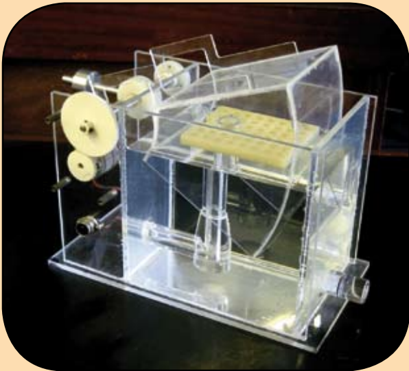
Wet wedge spirometer
