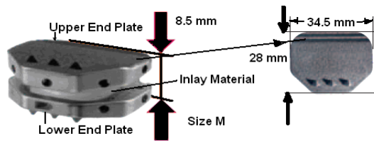
Fig. 1 Aesculap Activ-L™ Artificial Disc (size M)
