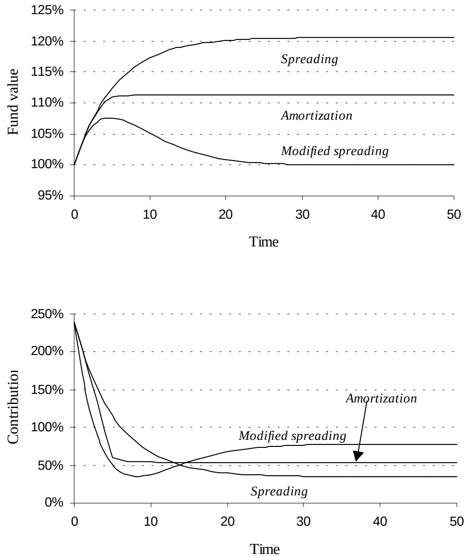
Figure 2: Fund value (per cent of actuarial liability) and contribution (per cent of normal cost) against time (years) when i_A = 1\% and i = 4.5\% for amortization, spreading and modified spreading.
