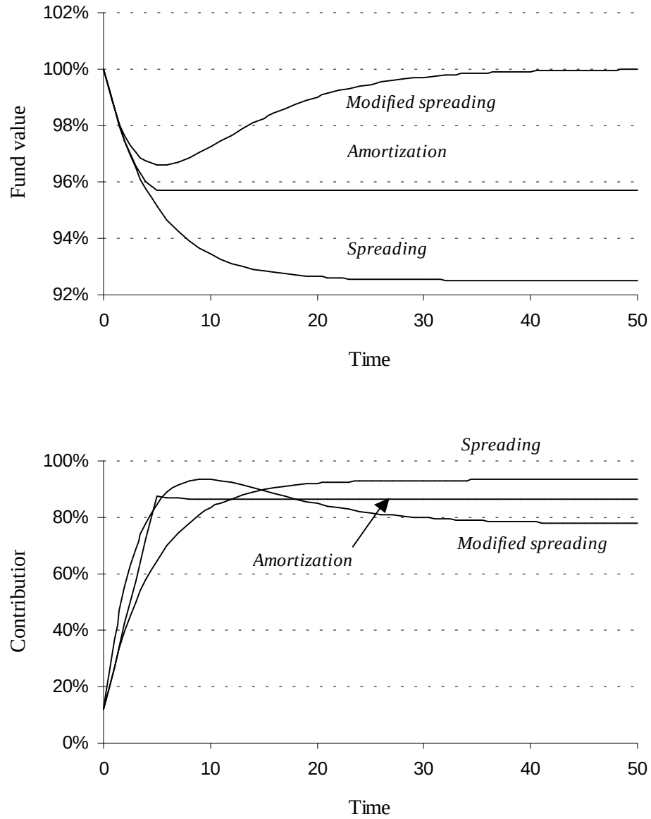
Figure 1: Fund value (per cent of actuarial liability) and contributor (per cent of normal cost) against time (years) when i_A = 6\% and i = 4.5\% for amortization, spreading and modified spreading.
