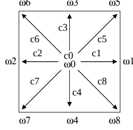
Figure 1: The standard two-dimensional 9-speed lattice ( D2Q9 ) used.
