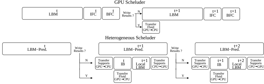
Figure 10: GPU (top) and heterogeneous CPU-GPU (bottom) implementations.
