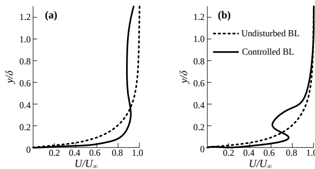
Figure 4 Boundary layer (BL) profiles controlled by MaVG (a) and MVG (b) (adapted from Holmes et al. [12]).
