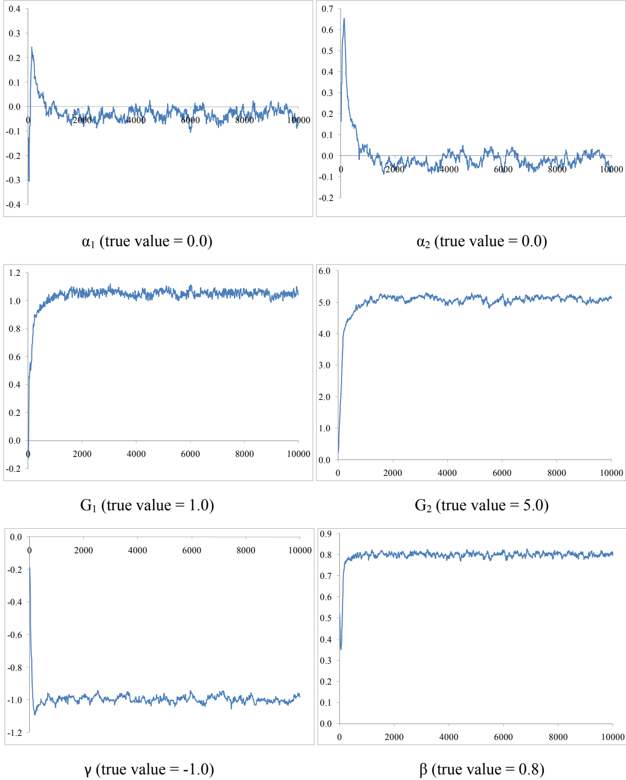
Figure 4: MCMC plots: Homogeneous Model with \beta = 0.8
