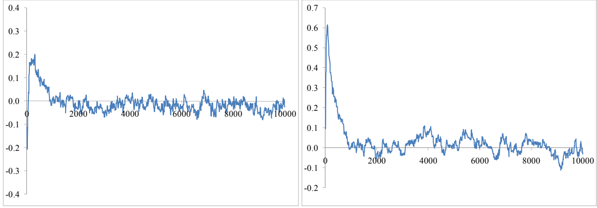
Figure 5: MCMC plots: Heterogeneous Model with \beta = 0.8
