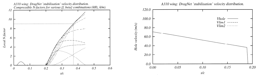
Figure 2 (a) Complete stabilisation of CF modes and (b) corresponding velocity distribution.
