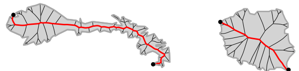
Fig. 5. The ratio between the longest path and the surface area gives a description of the compactness of a polygon. Both polygons are scaled to the same surface area.
