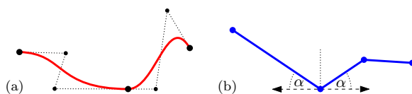
Fig. 4. (a) C^1 -continuous curves have a continuous derivative. The control points of consecutive curves line up. (b) Fixing the required tangent beforehand allows for a dynamic programming solution.
