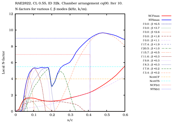
Figure 4 – Preliminary N-factor growth, transition x/c 0.409.
