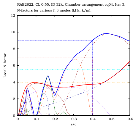
Figure 7 – Minimum configuration N-factor growth, transition x/c 0.401.
