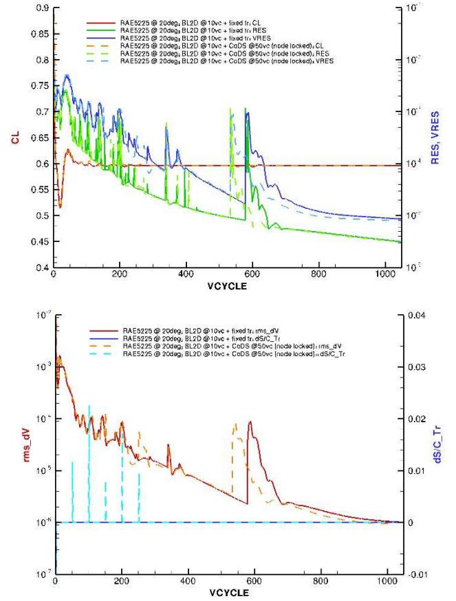
Fig. 4: RAE5225 swept at 20^\circ ; results for ‘stdb’ strategy (solid lines) compared with ‘lam1’ strategy (dashed).
