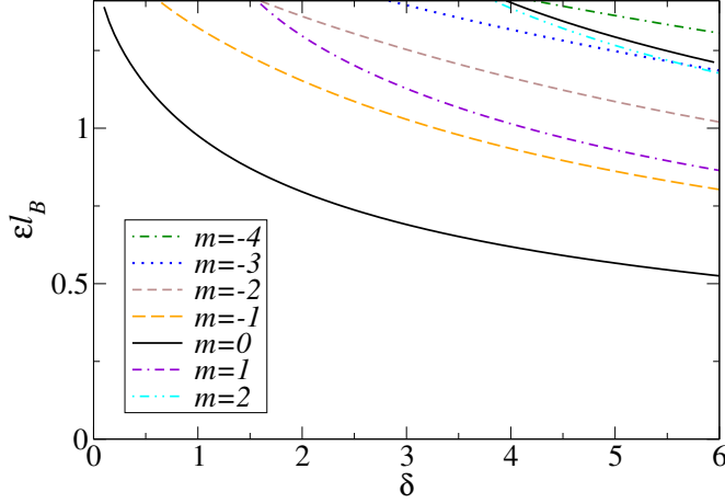
Fig. 3. (Color online) Low-energy eigenenergies (labeled by m ) for a disk-like magnetic quantum dot in graphene versus missing flux \delta = R^2/2l_B^2 .
