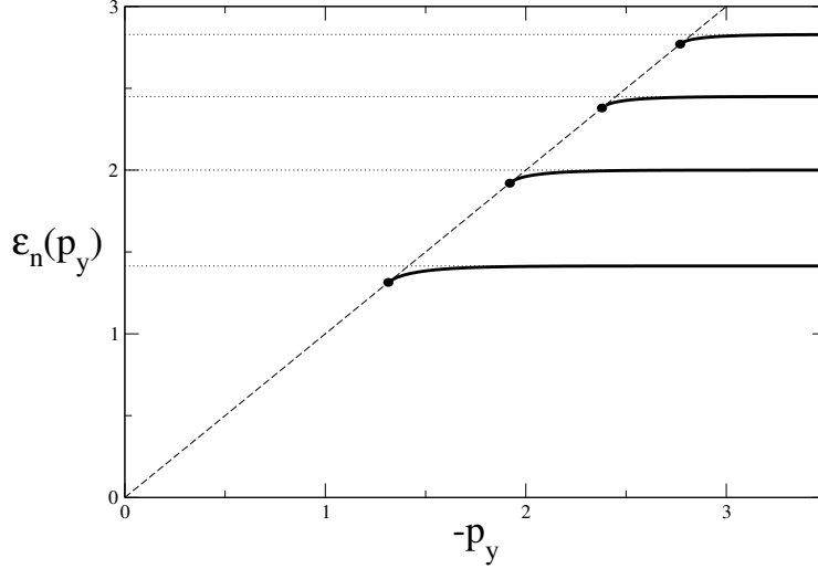
Fig. 2. Spectrum of the lowest-energy edge states. The momentum is expressed in units of l_B^{-1} and the energy in units of v_F/l_B . The dotted lines correspond to the relativistic bulk Landau levels \sqrt{2n} , with n positive integer.
