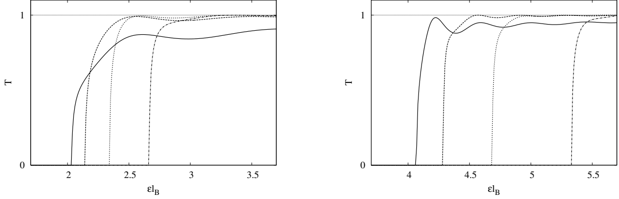
Fig. 1. Transmission probability for the magnetic barrier plotted as a function of the energy for two values of barrier width, d = 2l_B and d = 4l_B . The different curves correspond, from right to left, to the angles \phi = -n\pi/12 , with n = 2, 3, 4, 5 .
