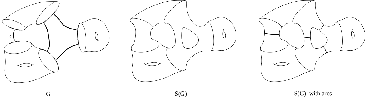
FIGURE 3. A prestable ribbon graph G and its associated surface S(G) . Note that the edge e itself forms a boundary component.
