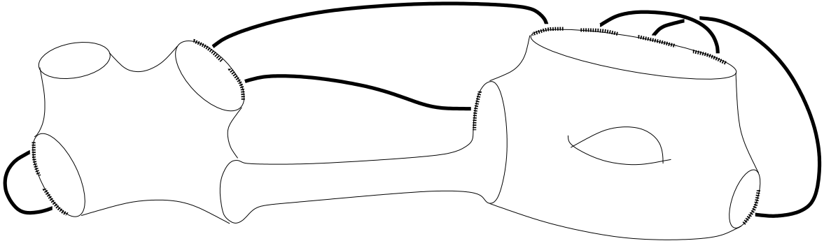
FIGURE 4. Graph obtained by ‘contracting’ the edge e in Figure 2.
