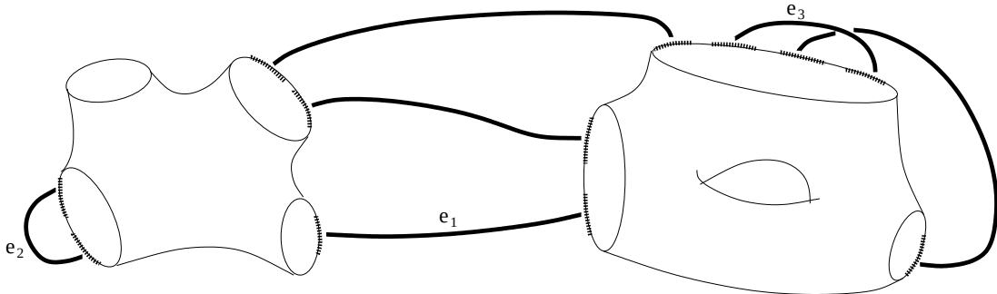
FIGURE 2. A prestable graph.
