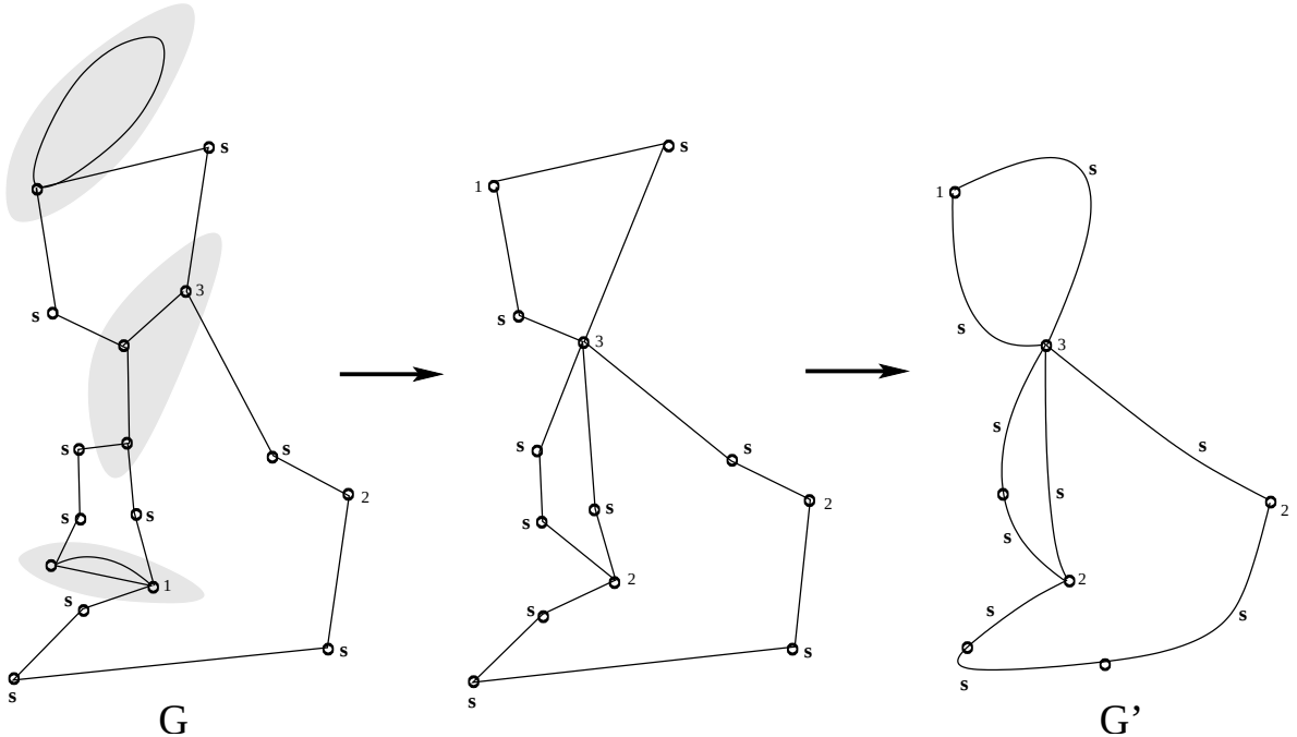
FIGURE 1. Contract edges connecting stable vertices, then replace unstable vertices by edges. Vertices are understood to have genus 0 unless otherwise noted.
