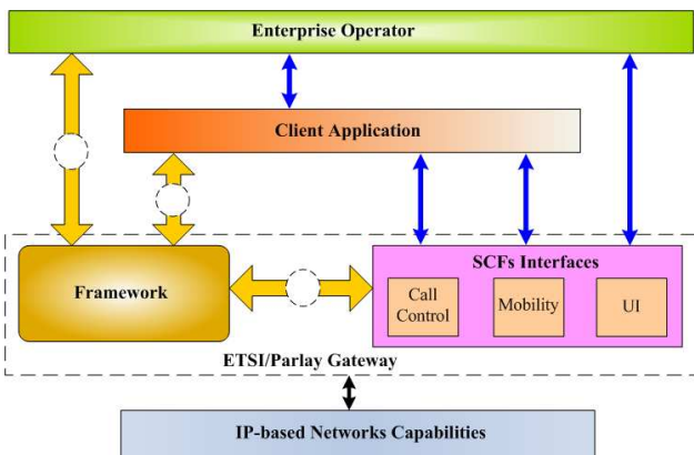
Fig. 1 The ETSI/Parlay Architecture
