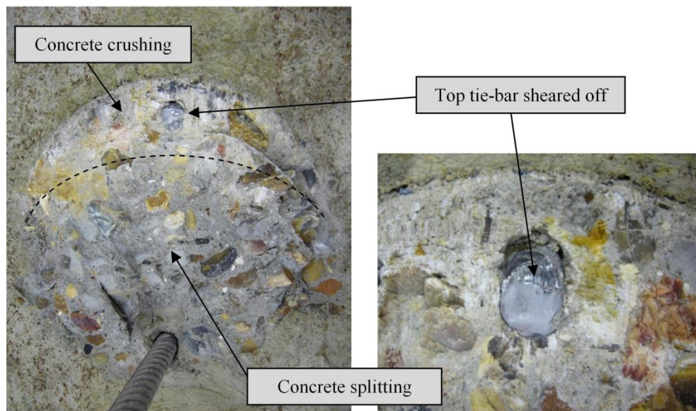
Fig. 22. Failure profiles of the tie-bar (Ø12mm) shear connection
