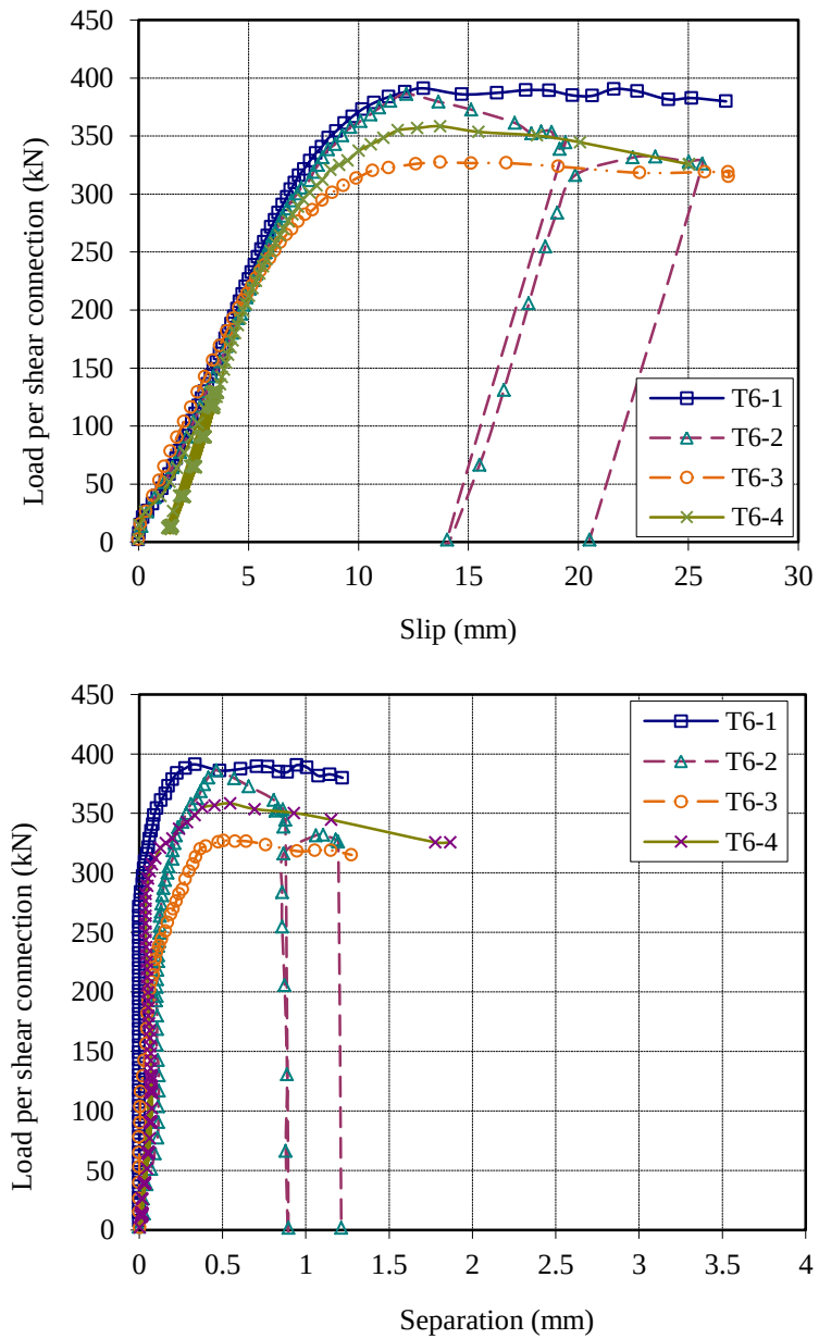
Fig. 17. Load-slip and load-separation curves of the tie-bar ( \varnothing 16\text{mm} ) shear connection in test group T6
