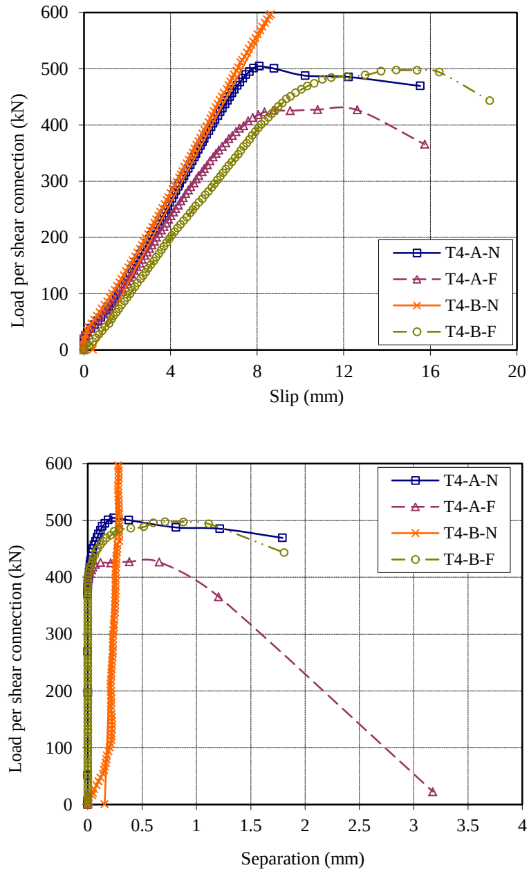
Fig. 15. Load-slip and load-separation curves of the web-welded shear connection in test group T4
