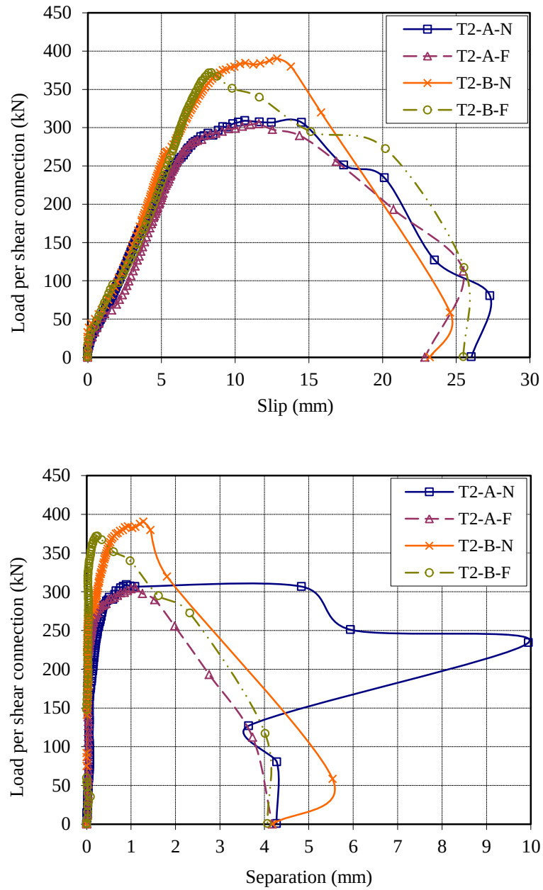
Fig. 13. Load-slip and load-separation curves of the tie-bar ( \varnothing 12\text{mm} ) shear connection in test group T2
