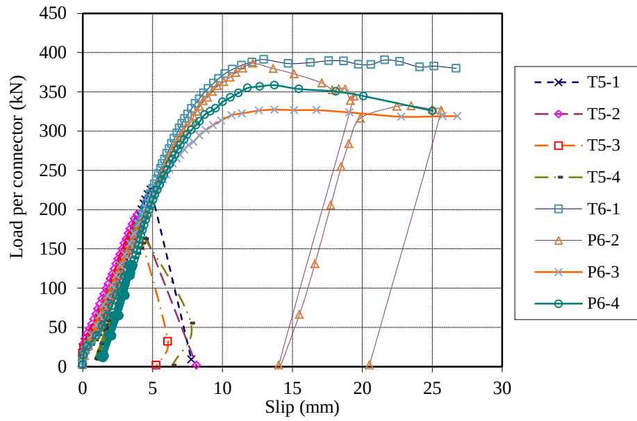
Fig. 18. Comparison of load-slip curves between concrete-infill-only (T5) and Ø16mm tie-bar (T6) shear connection
