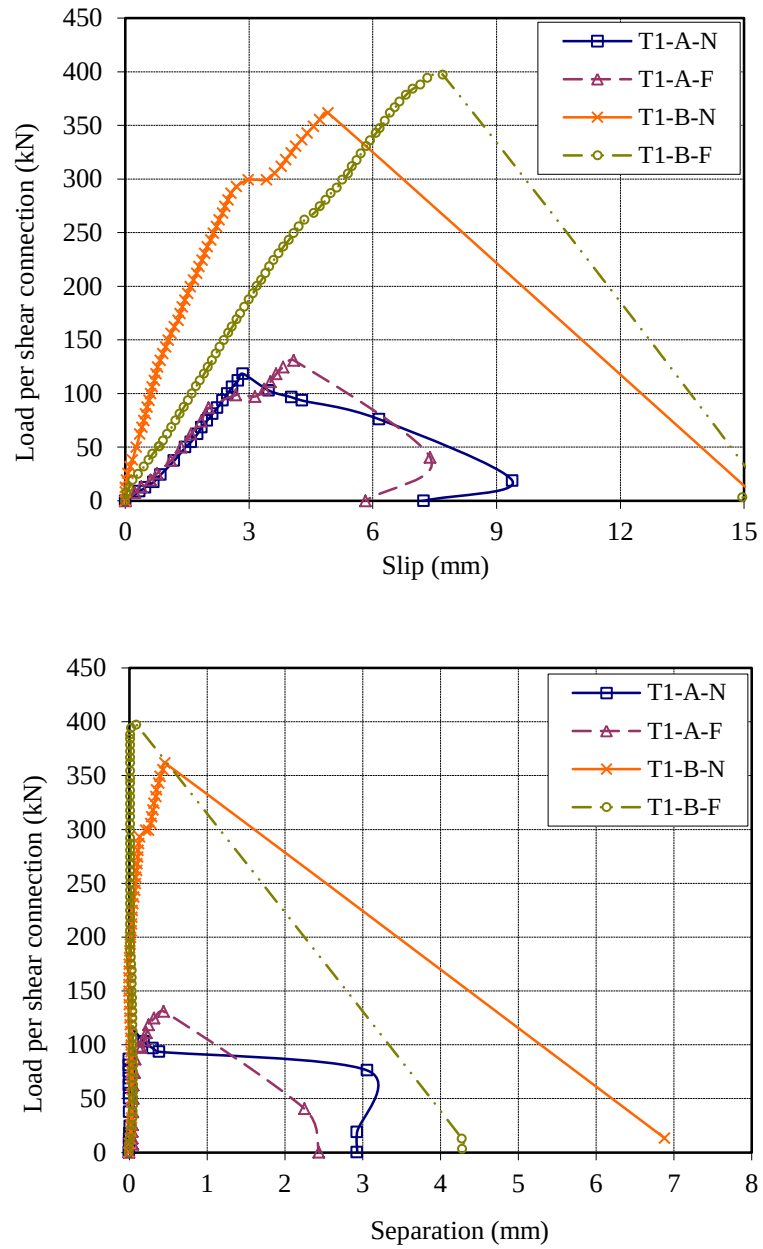
Fig. 12. Load-slip and load-separation curves of the concrete-infill-only shear connection in test group T1
