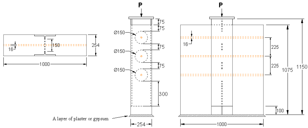
Fig. 10. Test specimen of test group, T6, tie-bar ( \varnothing 16\text{mm} ) shear connection
