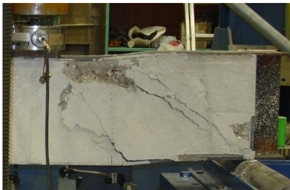
Fig. 10: USFB No.2 with concrete bursting
