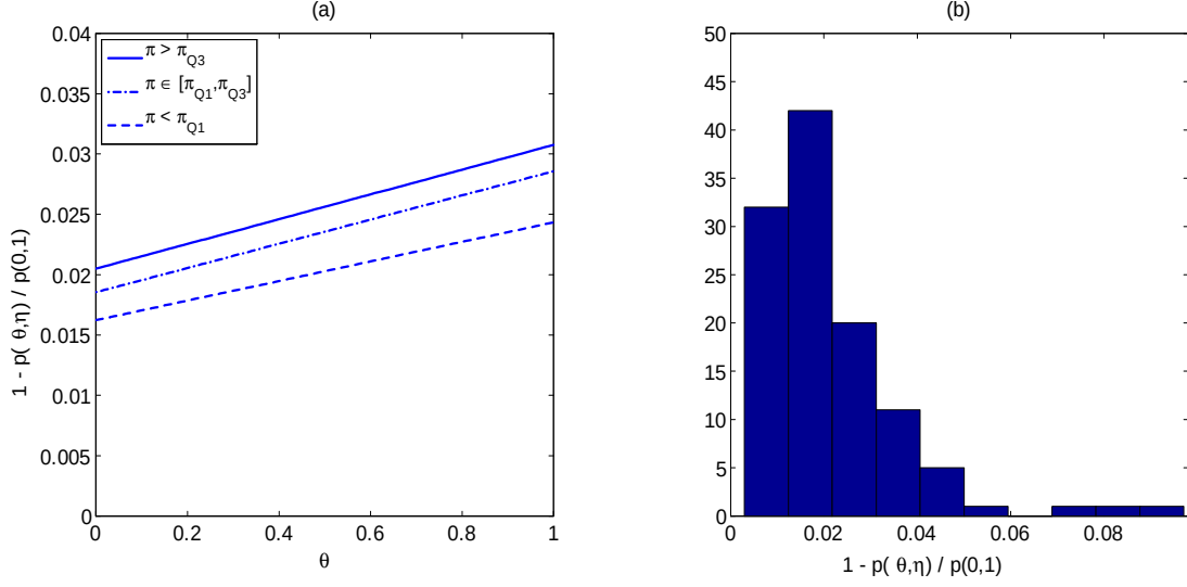
FIGURE 5: Predicted illiquidity-spillover discount of the dispersed shares, 1 - \frac{p(\theta, \eta)}{p(0, 1)} , for every value of \theta (panel (a)), and predicted histogram of the illiquidity spillover discount (panel (b)) evaluated at the predicted probability that the blockholder gets a liquidity shock, \theta_i , the predicted block liquidation parameter, \phi_i , and the predicted market thinness, \eta . The illiquidity-spillover discount function and histogram are constructed using the coefficients in Table III, specification (2).
