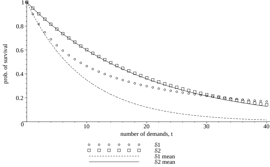
Fig. 3: The same two reliability functions as in previous figure, plus (as continuous lines for readability) reliability functions for hypothetical systems with pdf equal to the mean pdf s of S_1 and S_2 . The curves labelled S_2 and S_{2mean} are closer together than those labelled S_1 and S_{1mean} , which is intuitively explained by the probability distrib. of S_2 's pdf being narrower than that of S_1 's pdf . Also, the S_{2mean} curve lies completely below the S_2 curve, and the S_{1mean} curve below the S_1 curve, which holds in general by Thm. 1.
