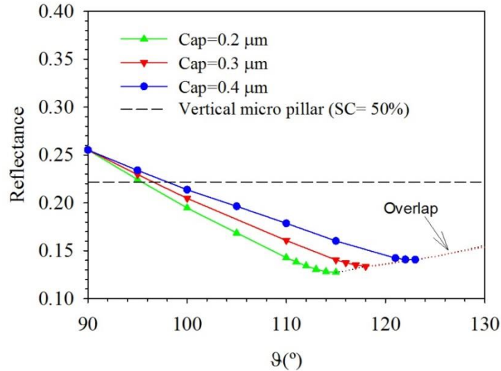
Fig. 6. Reflectance vs \theta at SC=30\% varying Cap size for H=1\text{ }\mu\text{m} .
