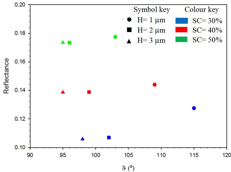
Fig. 7. Reflectance vs Optimum \theta for different values of H and SC with Cap = 0.2 \mu m .
