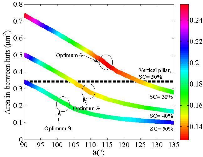
Fig. 3. Angular performance, Area in-between the huts vs \vartheta for H=1\text{ }\mu\text{m} , \text{Radiustop}=0.5\text{ }\mu\text{m} and \text{Cap}=0.2\text{ }\mu\text{m} where the line colour represents the R.
