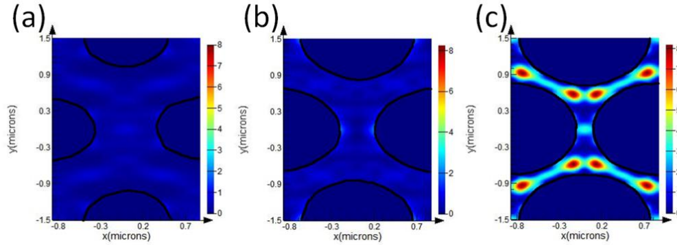
Fig. 4. Cross section showing E field intensity at 0.2\mu\text{m} above the substrate for structure with H=1\mu\text{m} , \text{Cap}=0.2\mu\text{m} and SC=30\% at \lambda \approx 0.373\mu\text{m} for (a): \vartheta=90^\circ . (b): \vartheta=105^\circ . (c): \vartheta=115^\circ .
