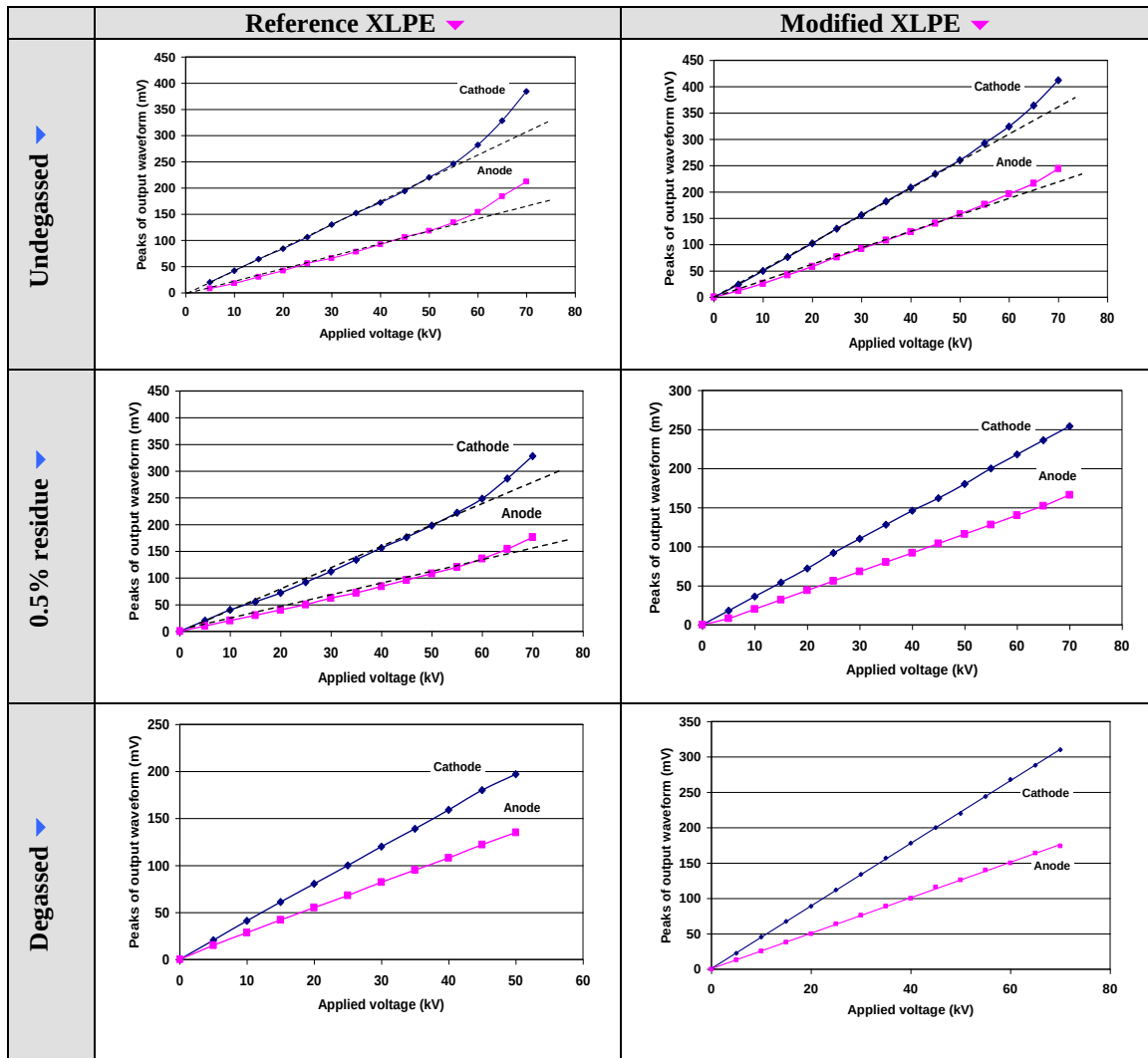
Figure 4. Relationship between the induced capacitive charge and the external voltage
