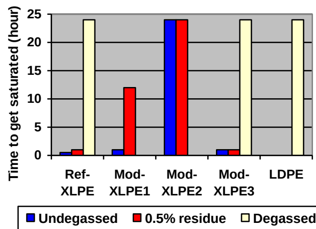
Figure 12. Saturation time of different samples
