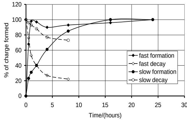
Figure 13. Space charge accumulation rate in accordance with decay rate
