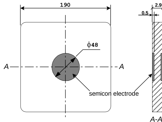
Figure 3. Sample dimension and its cross section
