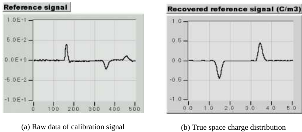
Figure 2. Space charge profile (in calibration) before and after attenuation and dispersion compensation
