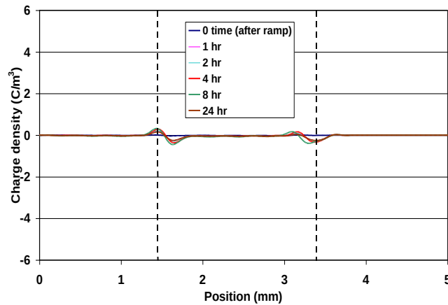
(c) Degassed sample with homocharge accumulation
