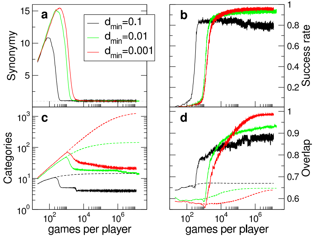
Figure 8. Results of simulations of the Category Game model with N = 100 and a flat (constant) d_{\min}(x) \equiv d_{\min} curve with different values of d_{\min} : a) Synonymy, i.e., average number of words per category; b) Success rate measured as the fraction of successful games in a sliding time windows games long; c) Average number of perceptual (dashed lines) and linguistic (solid lines) categories per individual; d) Averaged overlap, i.e., alignment among players, for perceptual (dashed curves) and linguistic (solid curves) categories.
