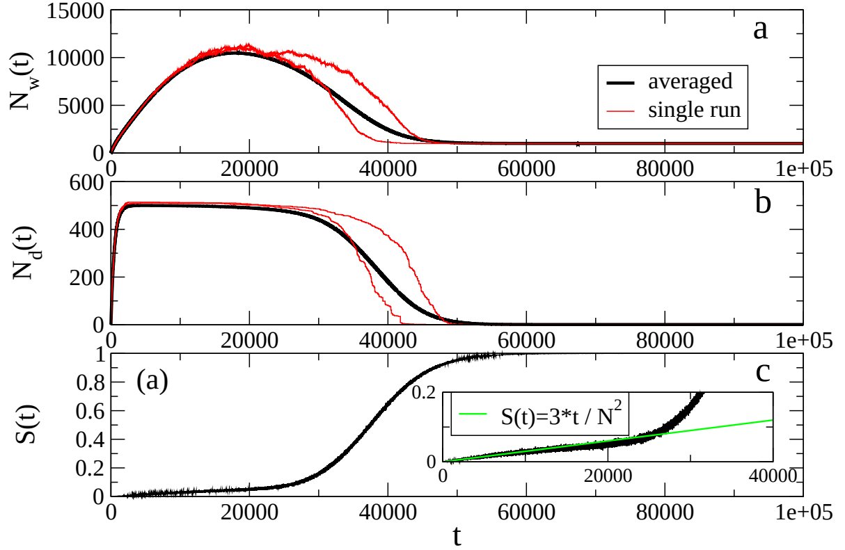
Figure 2. Naming Game. a) Total number of words present in the system, N_w(t) ; b) Number of different words, N_d(t) ; c) Success rate S(t) , i.e., probability of observing a successful interaction at time t . The inset shows the linear behavior of S(t) at small times. The system reaches the final absorbing state, described by N_w(t) = N , N_d(t) = 1 and S(t) = 1 , in which a global agreement has been reached.
