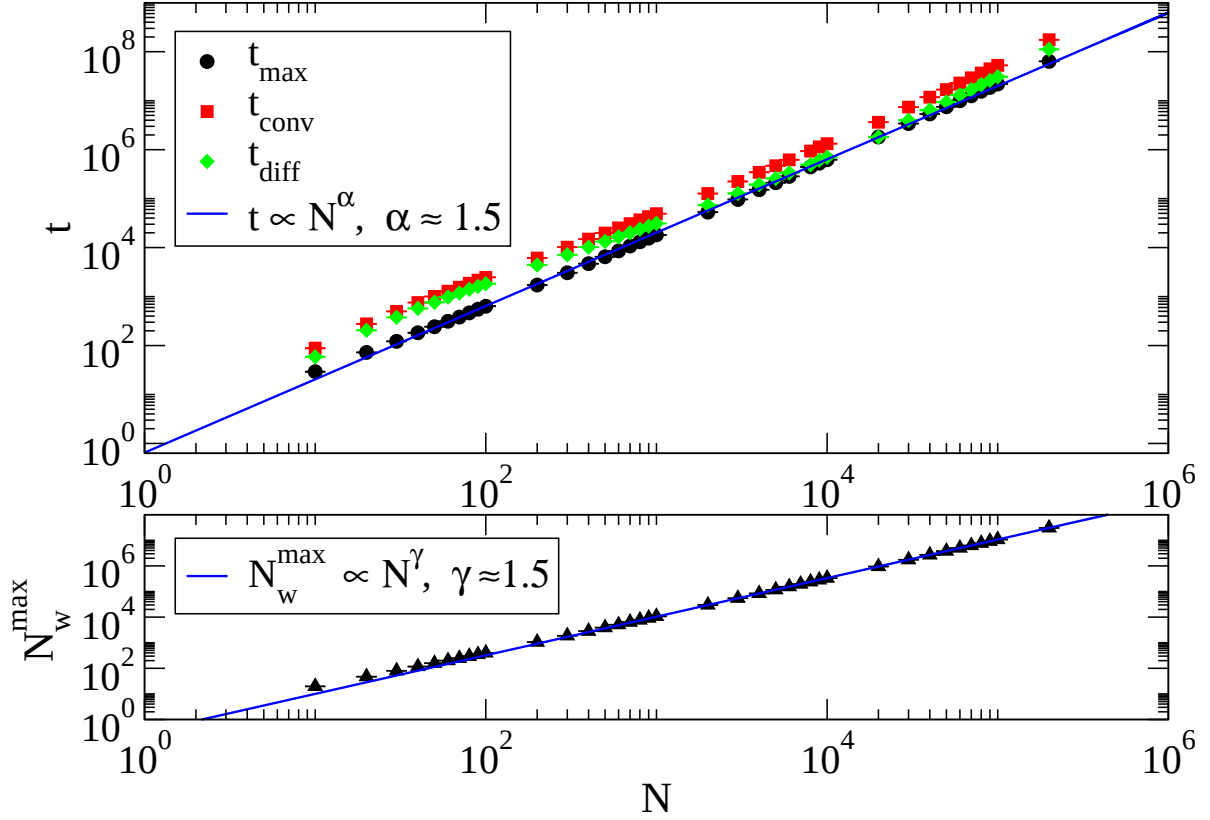
Figure 3. Naming Game. (Top) scaling of the peak and convergence time, t_{max} and t_{conv} along with their difference, t_{diff} . All curves scale with the power law N^{1.5} . (Bottom) the maximum number of words obeys the same power law scaling.
