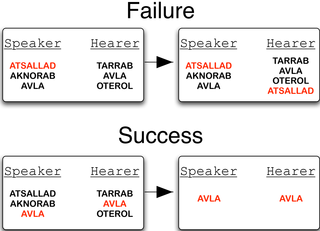
Figure 1. Naming Game. Examples of the dynamics of the inventories in a failed (top) and a successful (bottom) game. The speaker selects the word highlighted. If the hearer does not possess that word he includes it in his inventory (top). Otherwise both agents erase their inventories only keeping the winning word (bottom).
