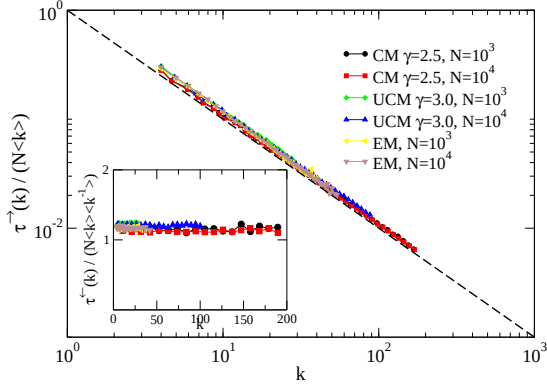
FIG. 10: (Color online) Reduced MFPTs as a function of the degree k for looped complex networks. We recover the simple mean-field predictions \tau_L^-(k) \simeq \langle k \rangle N / k (main figure) and \tau_L^-(k) \simeq \langle k \rangle \langle k^{-1} \rangle N (inset).
