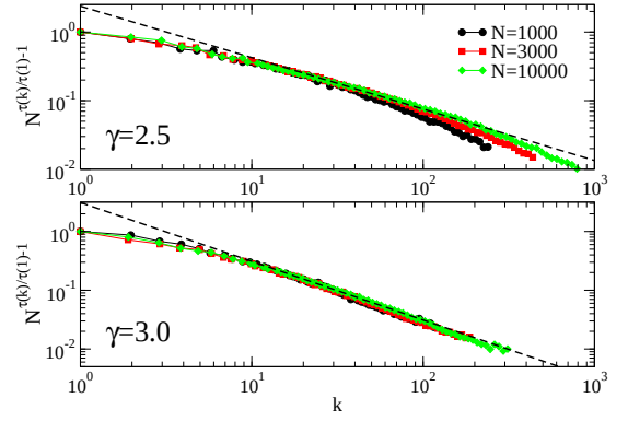
FIG. 14: (Color online) Rescaled MRTT \bar{\tau}_T(t) as a function of the source degree k and for randomly chosen targets in SF trees. Predictions of Eq. (30), i.e. N^{\tau(k)/\tau(1)-1} \bar{\tau}(k) \sim k^{(1-\gamma)/2} , are plotted as dashed lines.
