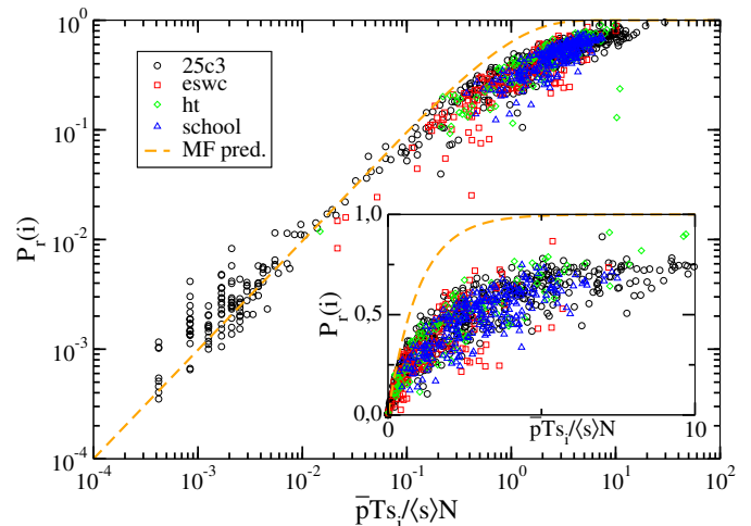
Figure 12. (Color Online) Correlation between the probability of node i to be reached by the RW, P_r(i) , and the rescaled strength \bar{p}Ts_i/N\langle s \rangle for different datasets. The curves obtained by different dataset collapse, but they do not follow the mean-field behavior predicted by of Equation (17) (dashed line). The inset shows the same data on a linear scale, to emphasize the deviation from mean-field.
