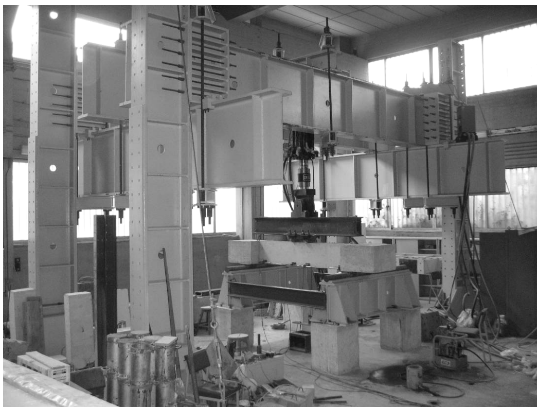
Fig. 6. Experimental set-up
