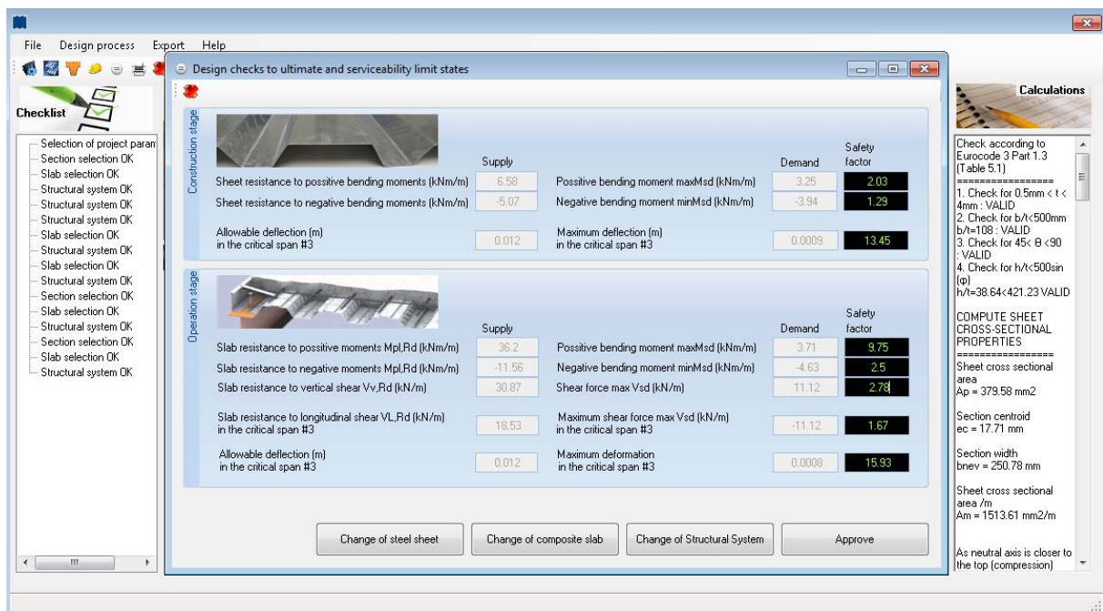
Figure 18. Final design check against serviceability and ultimate limits states.
