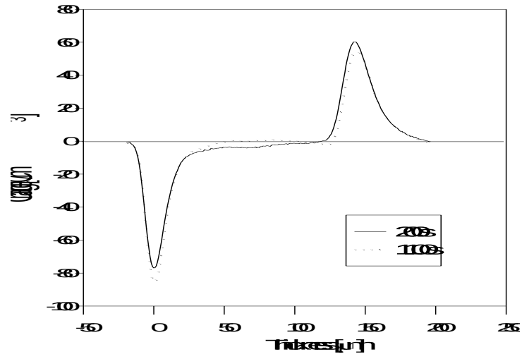
a-Charge profiles relevant to poling field of 80 kV/mm
