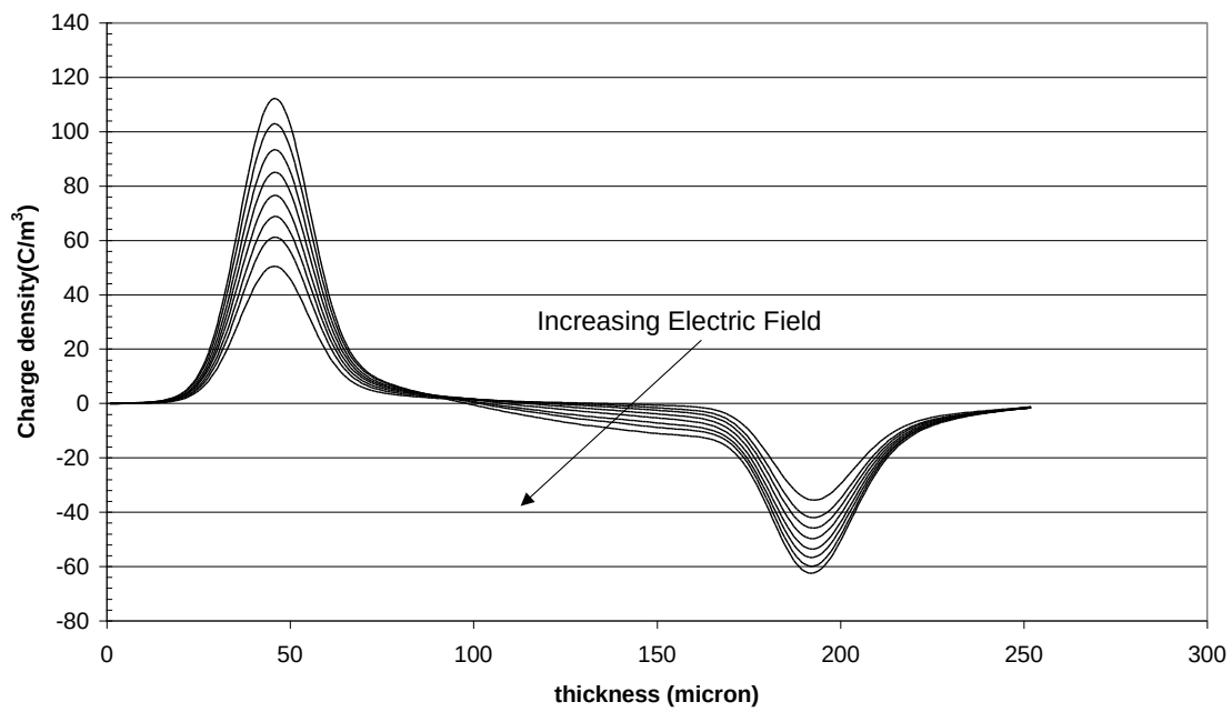
Figure 15: Charge profiles at different fields for a progressive DC stress test (Cable C)
