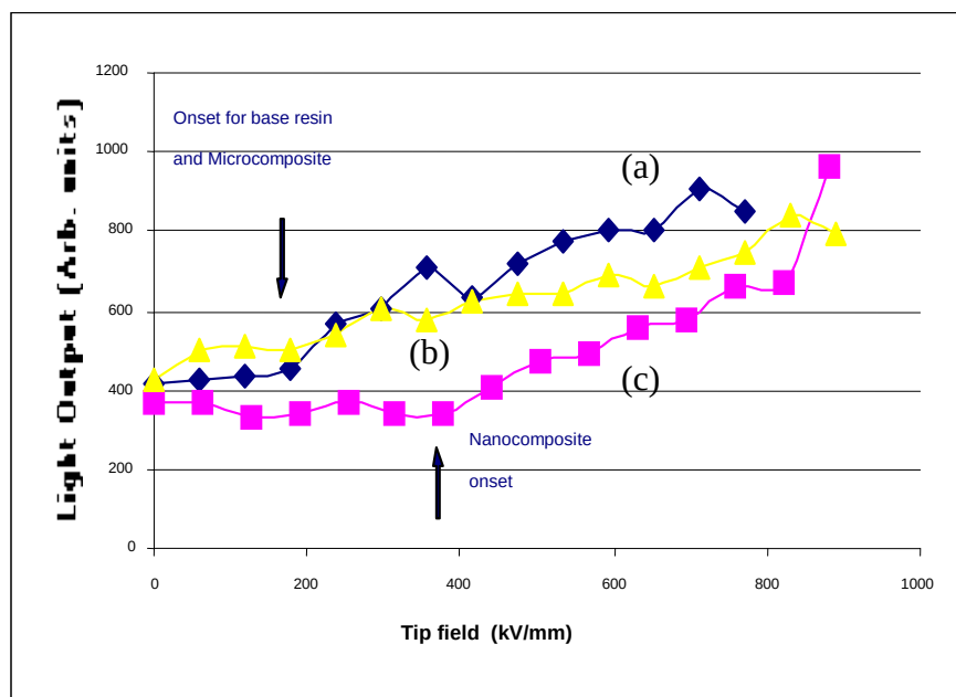
Figure 8. Electroluminescence characteristics in \text{TiO}_2 composites. (a) base resin, (b) 10% micro (c) 10% nano.
