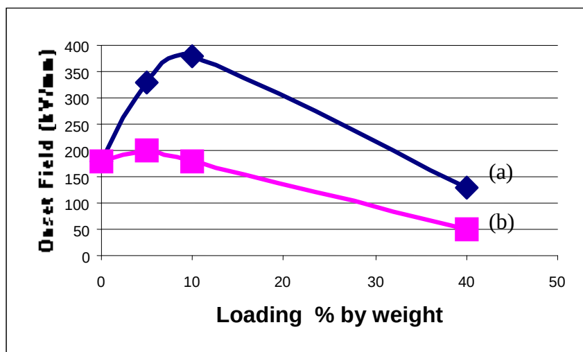
Figure 9. Electroluminescence onset field as a function of \text{TiO}_2 loading. (a) 23 nm, (b) 1.5 \mu\text{m}
