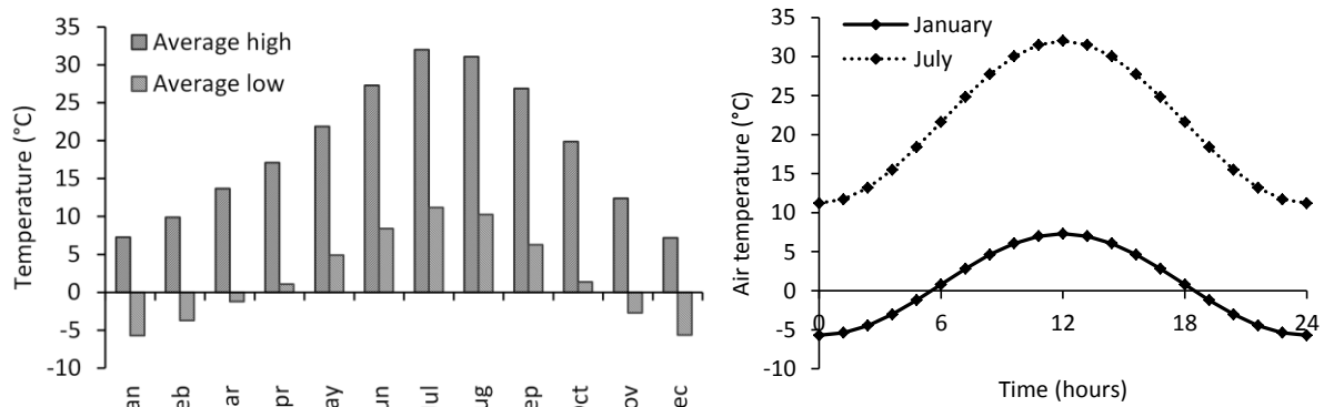
Figure 2: Monthly average maximum and minimum air temperatures in Nevada USA, and examples of assumed daily sinusoidal variation of air temperature
