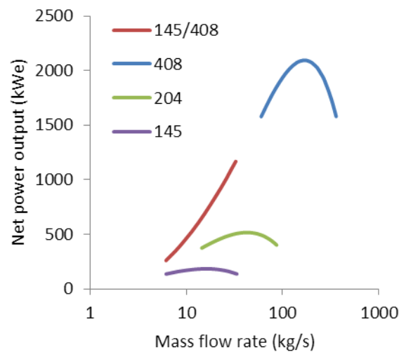
Figure 7: Net power output from TFC system using single and two-stage expanders
