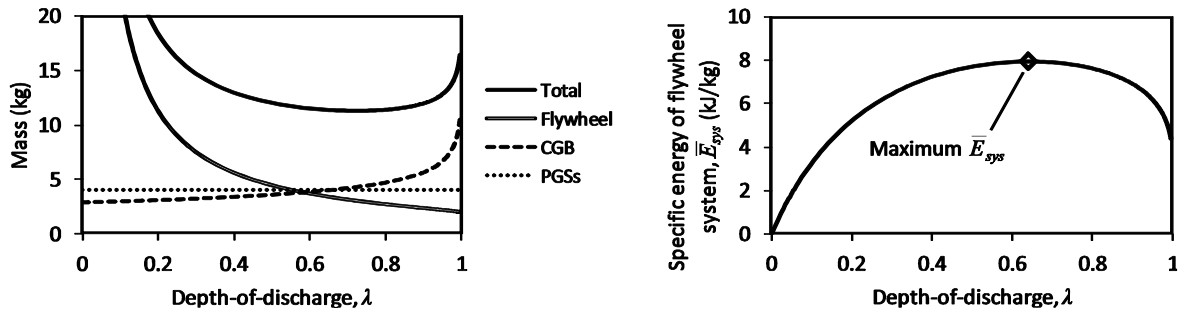
Figure 17 – Mass of components and specific energy of flywheel system as functions of \lambda using a 2-PGS, 4-CGB transmission for the passenger car application defined in Table 1
