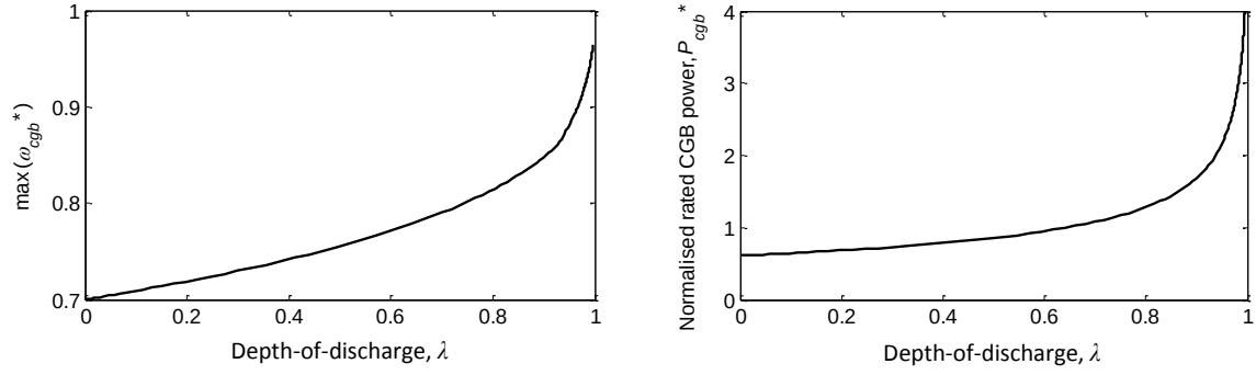
Figure 16 – Variation of \max(\omega_{cgb}^*) and P_{cgb}^* as functions of \lambda for 2-PGS, 4-CGB transmission with G_1 = 0.25
