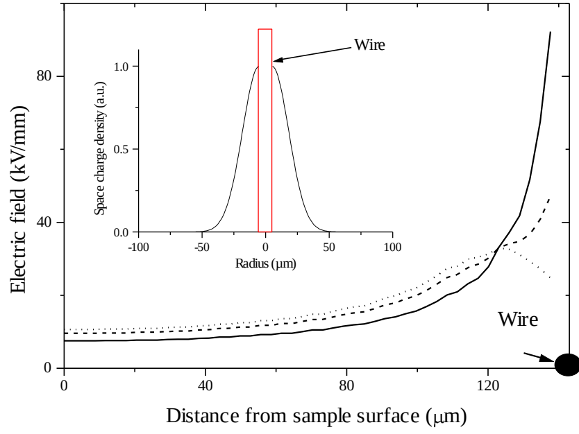
Figure 9 : Space charge field for different space charge density. Solid line : \rho = 0 , dashed lined : \rho = 50 \text{ C.m}^{-3} , doted line : \rho = 75 \text{ C.m}^{-3}
