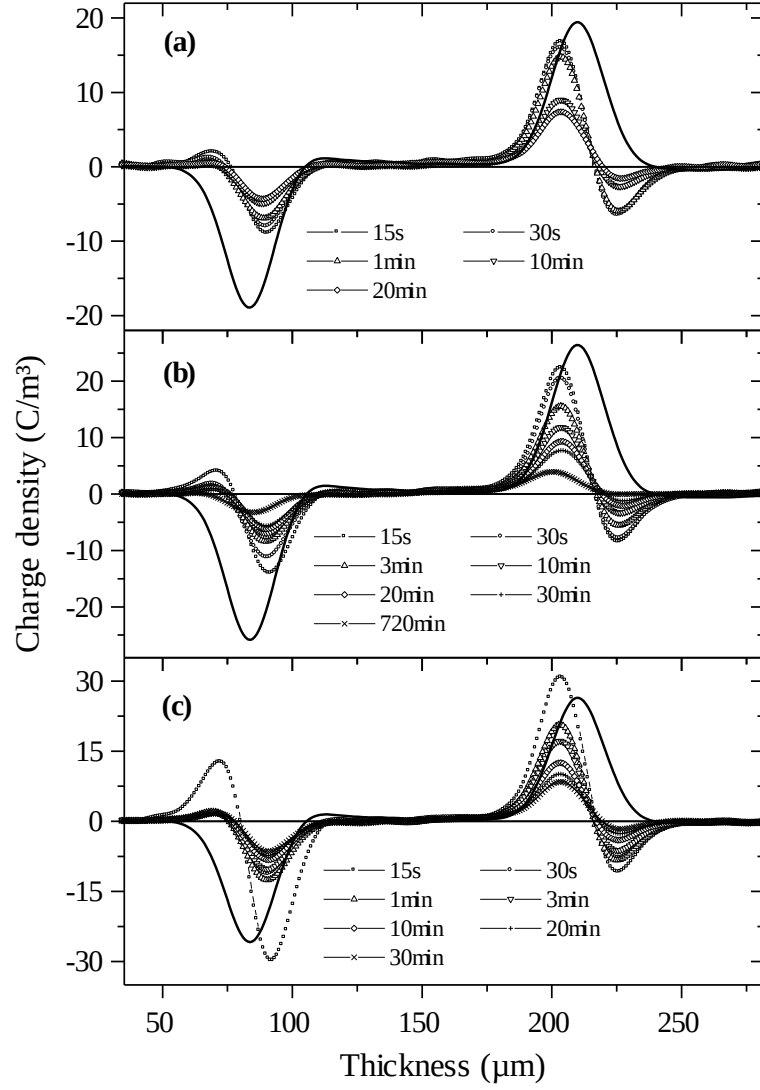
Figure 14: Space charge profiles for different fields : (a)-72 kV/mm, (b)-100 kV/mm and (c)-130 kV/mm. The solid line is the Volt-on signal (Y-scale \times 0.2 ) measured at the end of the polarization period. The volt-off profiles were obtained at different times as indicated. Cathode on the left, anode on the right.
