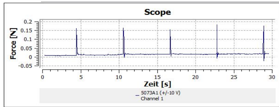
Figure 5.16 Oscilloscope reading for GM material
