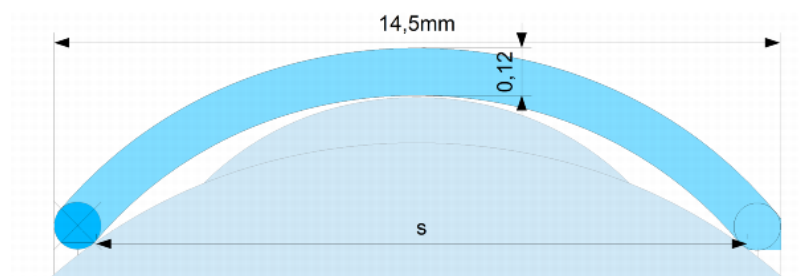
Figure 6.5 "Aligned" fit of a soft contact lens (not to scale).
