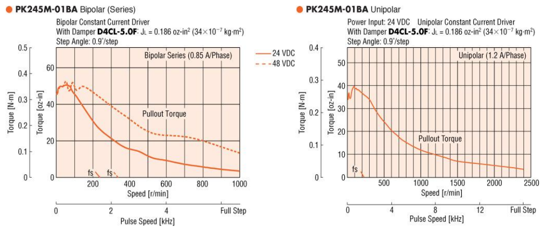
Figure 5.5 Torque graphs for stepper motor
