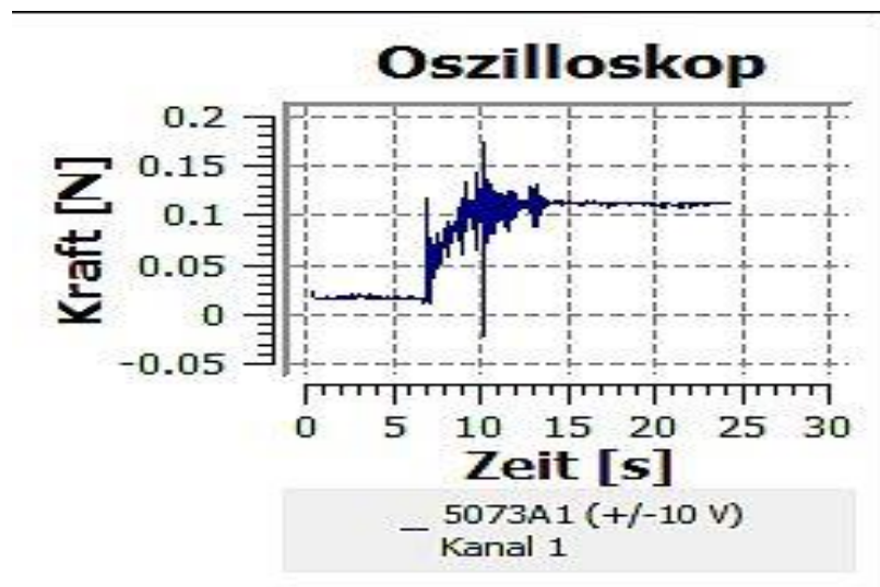
Figure 5.11 Oscilloscope display during sensor calibration between 'no force applied' and 'force applied'.
