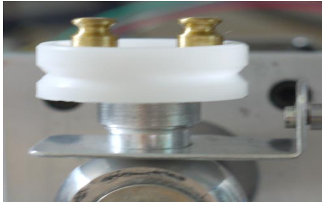
Figure 5.12 10g total force on top of the substrate aluminium substrate and aluminium sample.
