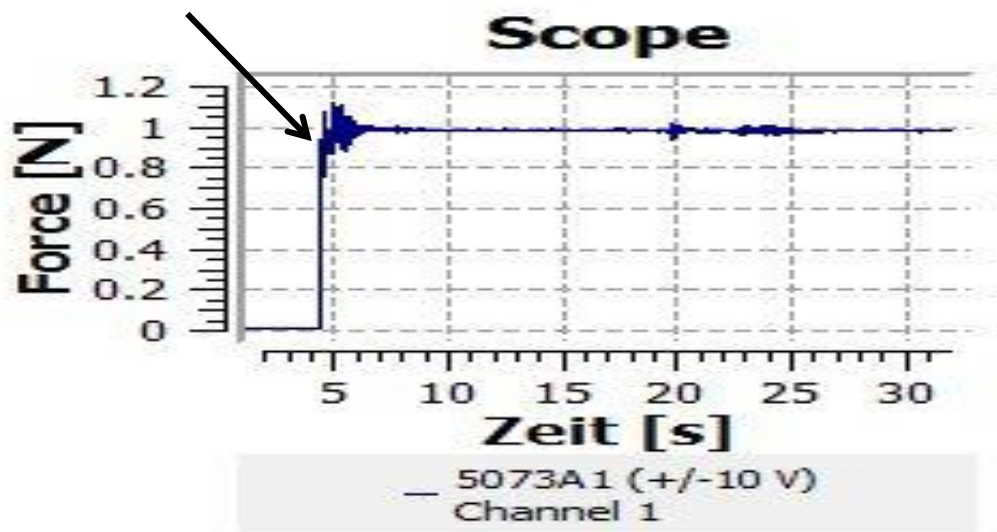
Figure 5.13 Example reading of static friction.
