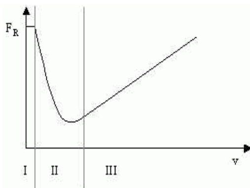
Figure 4.2 A schematic Stribeck curve showing the three different friction phases.
