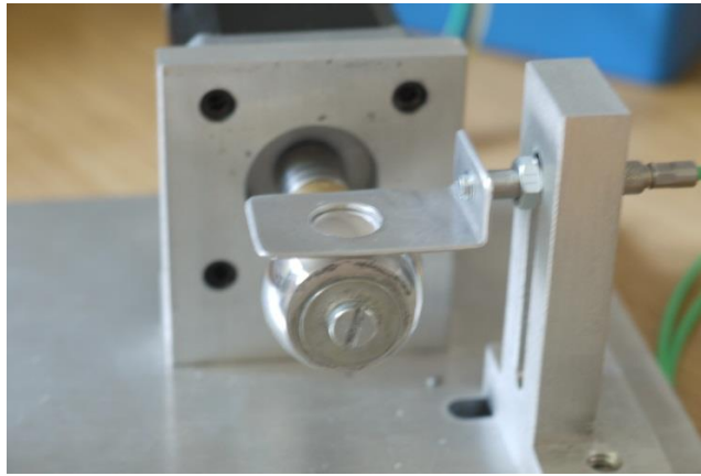
Figure 5.3 Tribometer base showing the substrate attached to the stepper motor and the disc holder
