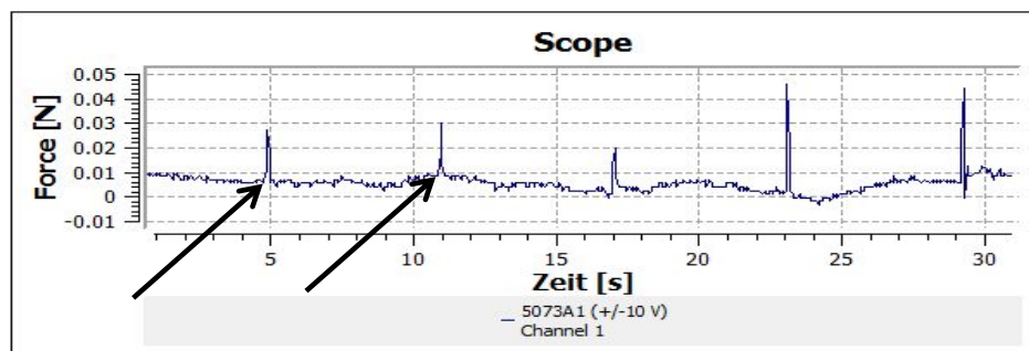
Figure 5.17 Oscilloscope reading of Definitive material at mixed friction 10
