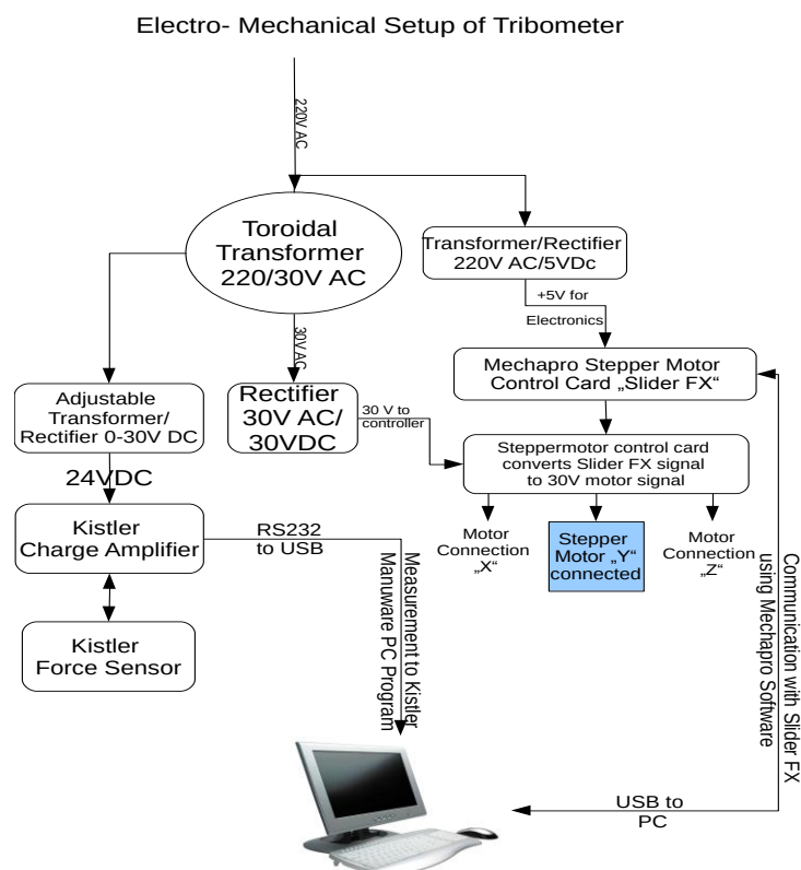
Figure 5.1 Tribometer Schema to show how the different components of the tribometer apparatus are connected to the Tribometer Base
