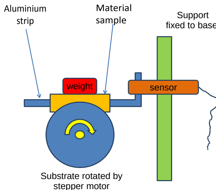
Figure 5.2 Tribometer set up.
