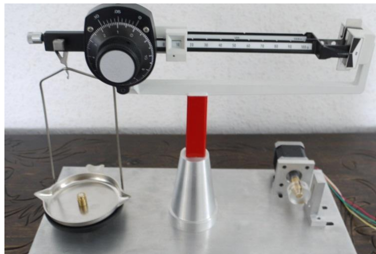
Figure 5.4 Tribometer balance attached to base.
