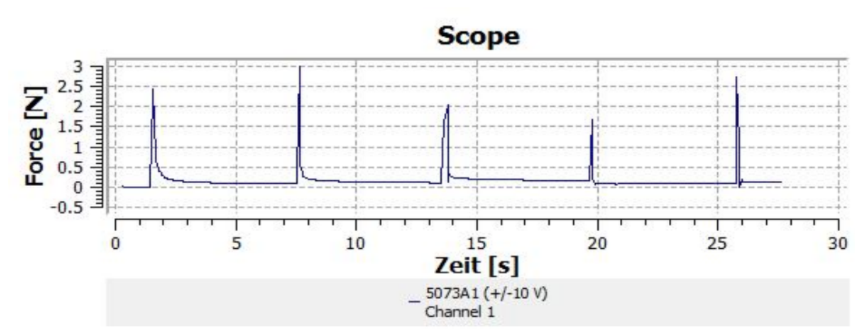
Figure 5.14 Oscilloscope reading for HEMA (V38) material - unlubricated friction.
