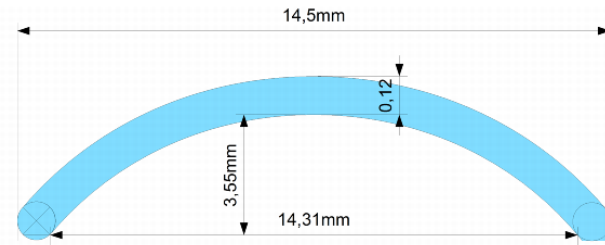
Figure 6.4 Section of a monocurve contact lens with effective inner lens diameter
