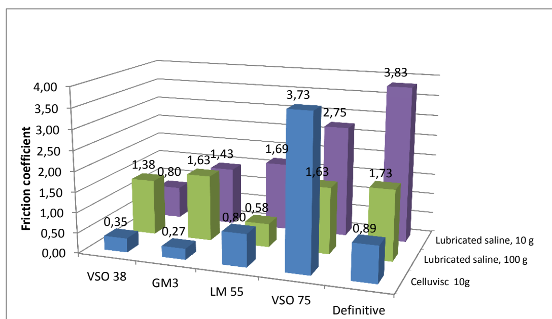
Figure 8.1 Average coefficients of friction in ascending order
