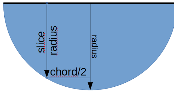
Figure 4.12 Explanation for the calculation of the slice diameter of a sphere (spatial diameter) Note: the diameter is 2 times the radius.
