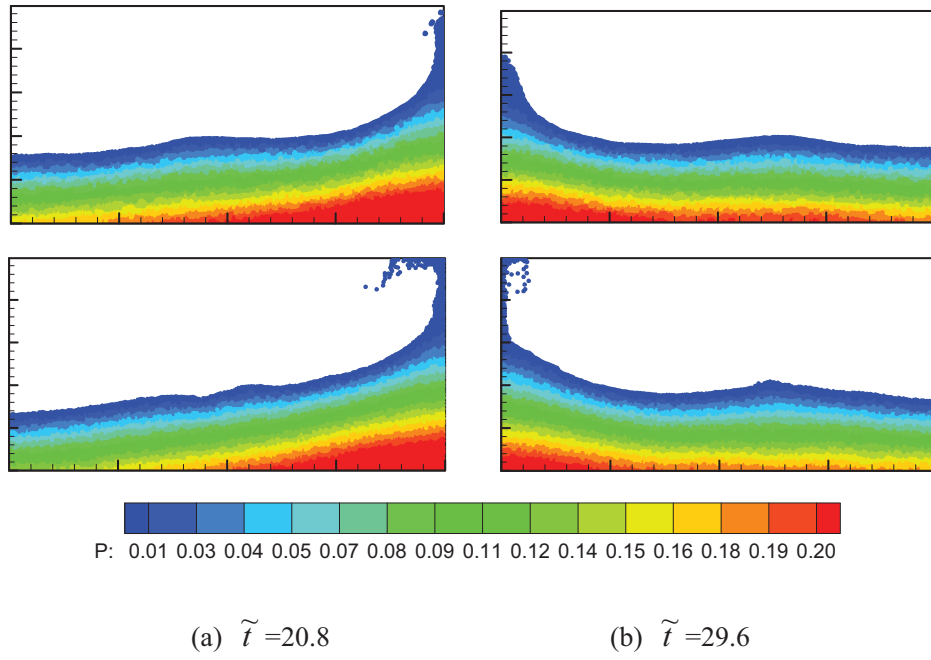
Fig. 22 Snapshots of pressure distribution of violent sloshing compared: CISPH2 (upper row) and ISPH_R (lower row)
