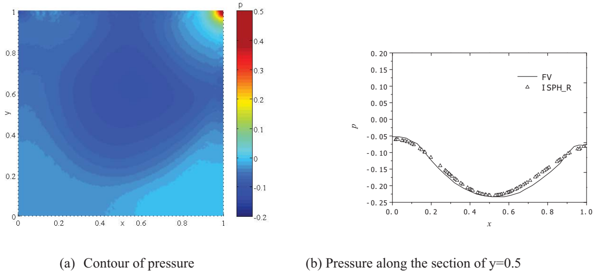
Fig. 25 Pressure of lid-driven cavity flow
