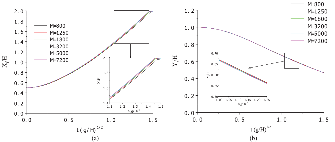
Fig. 7 Comparison of (a) water fronts represented by X_f and (b) water column heights represented by Y_t corresponding to different particle numbers
