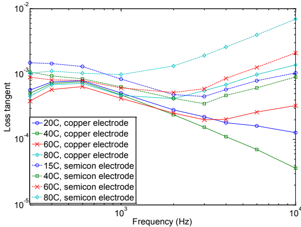
Figure 9 Comparison of the results from different sample preparation methods. (copper electrode: solid lines, semicon electrodes: dotted lines)
