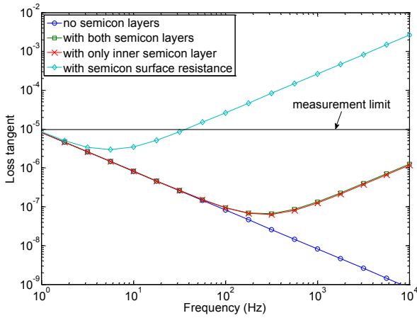
Figure 8 Modelling results on the effect of semicon shields
