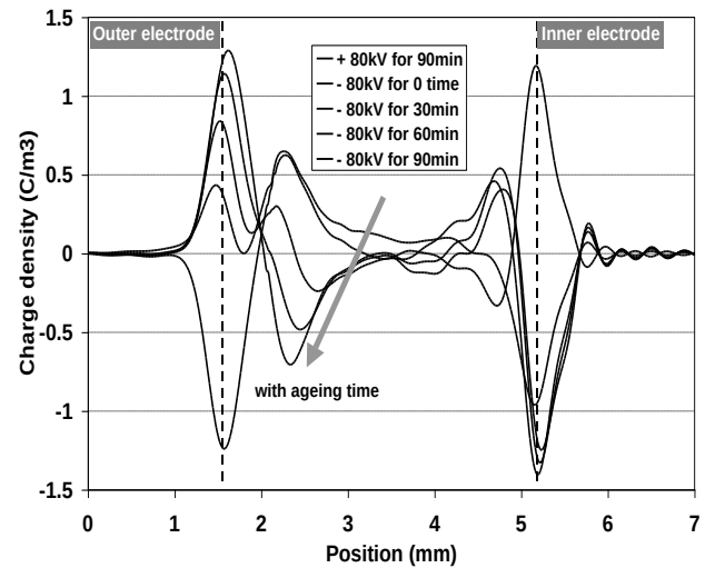
(c) Space charge accumulation with reversed voltage application time
