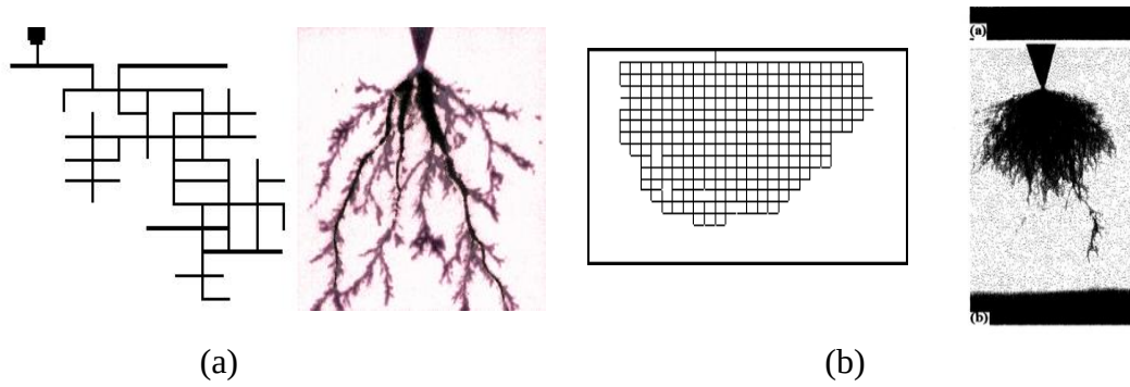
Figure 3 Comparison of tree structures from the model and experimental electric trees: (a) branched trees; (b) bush trees
