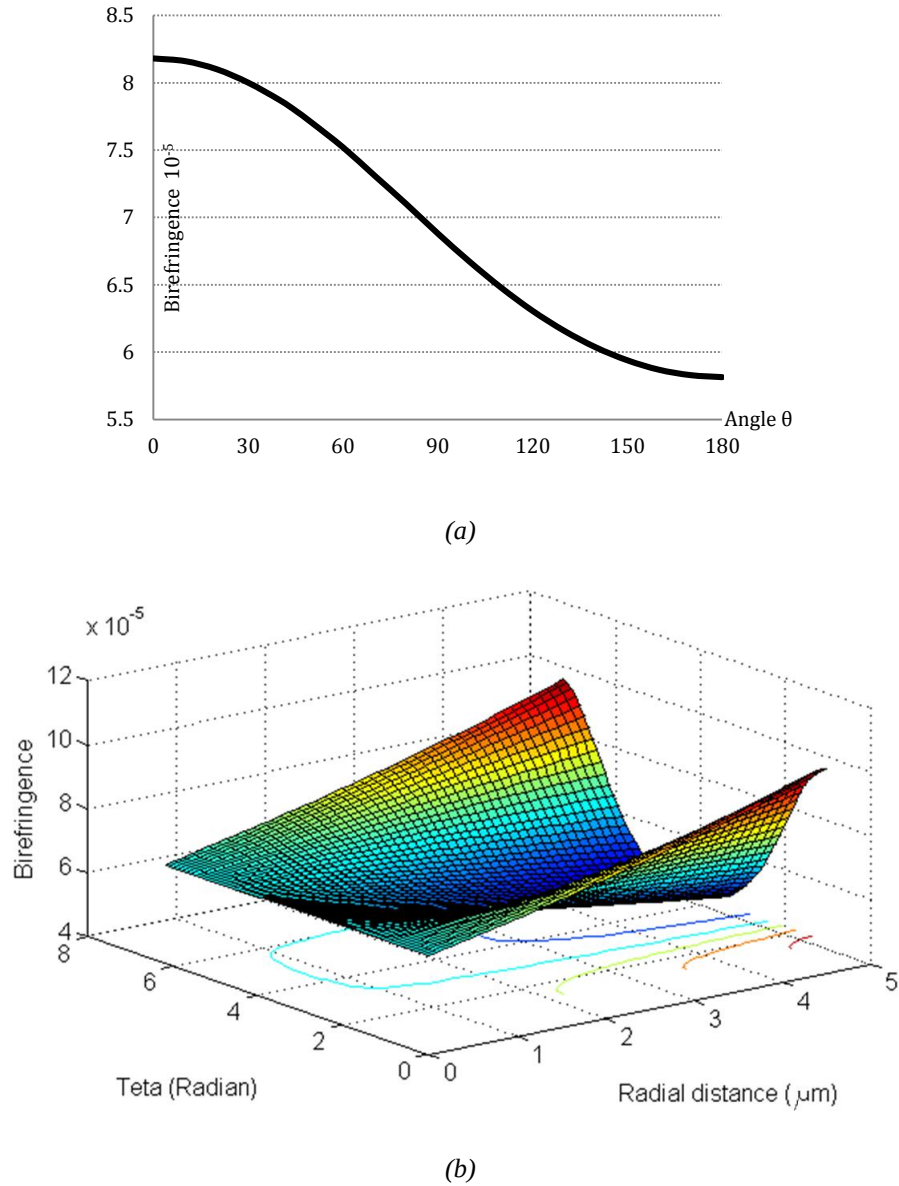
Figure 3.15. Birefringence distribution in a one-hole fibre core as a function of angles \theta . (a) Edge of the core. (b) Cross section of the core
