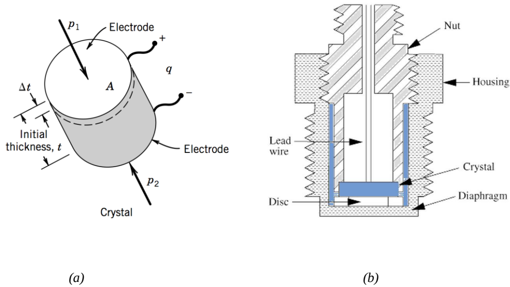
Figure 2.7 Piezoelectric pressure transducer using a diaphragm as a force-summing device (a) Schematic of pressure transducer (b) incorporating the diaphragm in the housing [42]
