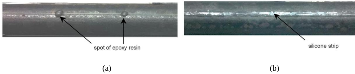
Figure 5.3 (a) Instrumented rebar with unprotected sensor. (b) Instrumented rebar with sensor protected by a thin layer of silicone.
