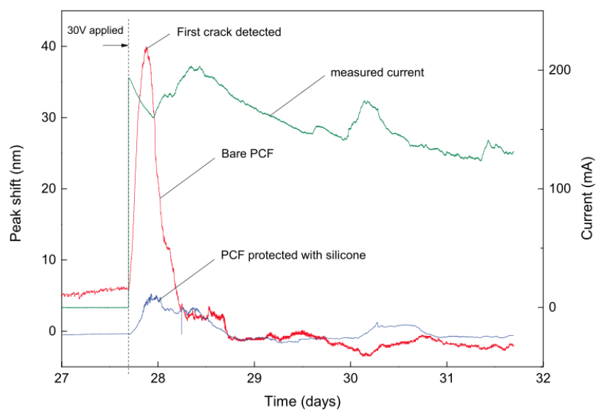
Figure 5.6. Behaviour of bare and silicone-protected PCFs under accelerated corrosion (Rebar 2).
