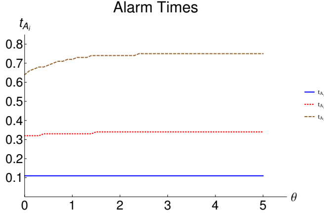
Figure 3.2: First 3 alarm times t_{A_1}, t_{A_2}, t_{A_3} under a system with multiple alarms, based on Example 3.2.4. Parameter values: \lambda = 1 , \alpha = 5 , \beta = 2 , u_0 = 5 , c = 10 , \Delta u = 1 , a = 0.4 , b = 0.03 , d = 2 and y = 0.5 . Blue (solid), red (dotted) and brown (dashed) lines represent alarm times 1, 2, 3, respectively.
