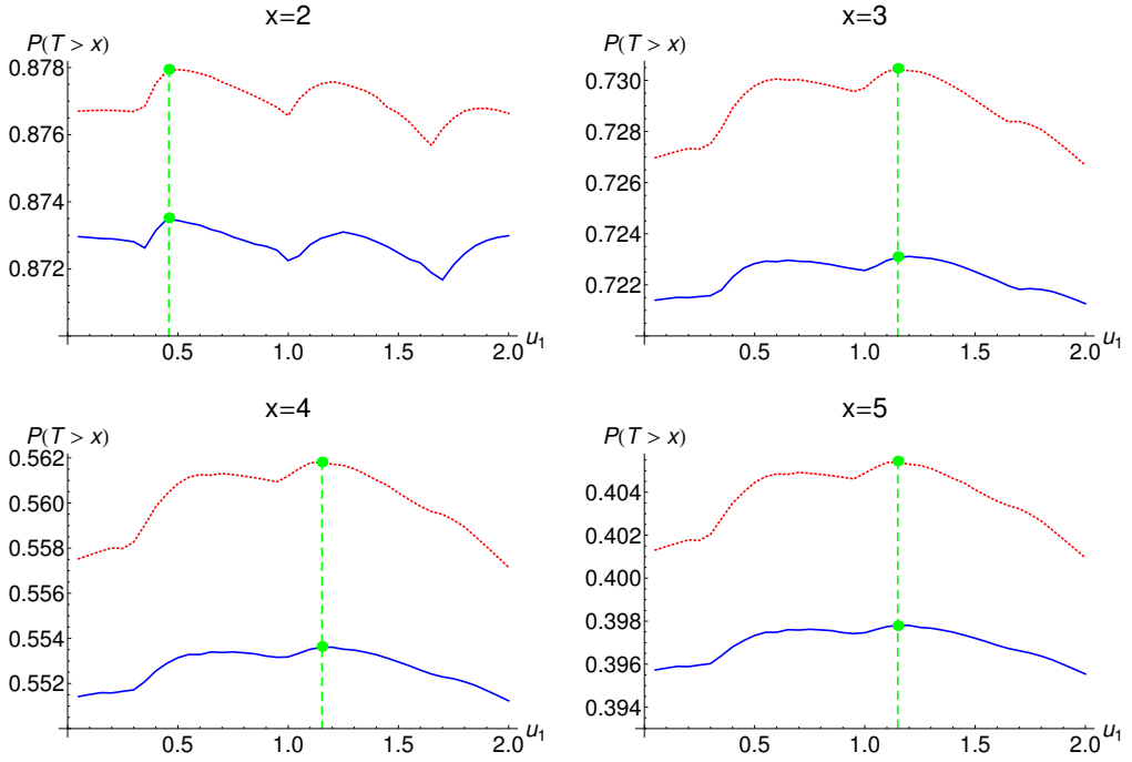
Figure 3.6: Survival probability P(T > x) against different choices of u_1 . Parameter values: \lambda = 2 , \alpha = 0.7 , u_0 = 10 , u' = 2 , c = 1 , a = 0.4 , b = 0.25 and d = 4 . Blue (solid) and red (dotted) lines represent r = 5\% and r = 10\% respectively.
