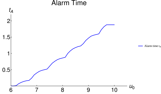
Figure 3.3: Alarm time t_A for varying choices of initial capital u_0 . Parameter values: \lambda = 2 , \alpha = 0.7 , u = 10 , c = 1 , a = 0.4 , b = 0.25 and d = 3 .
