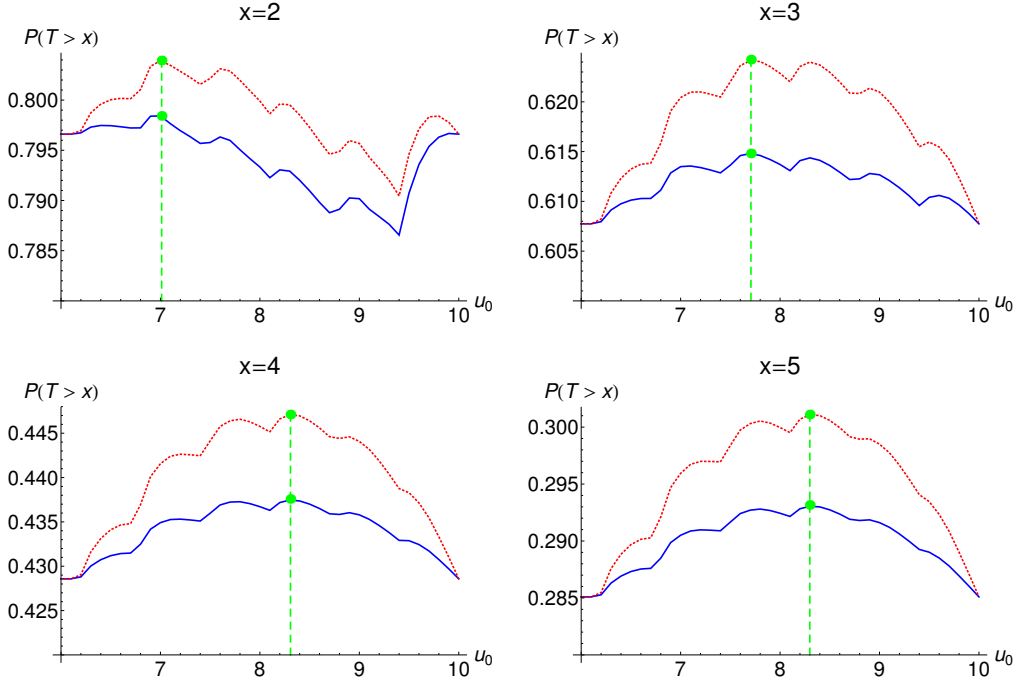
Figure 3.4: Survival probability P(T > x) against different levels of initial capital u_0 . Parameter values: \lambda = 2 , \alpha = 0.7 , u = 10 , c = 1 , a = 0.4 , b = 0.25 and d = 3 . Blue (solid) and red (dotted) lines represent r = 5\% and r = 10\% respectively.
