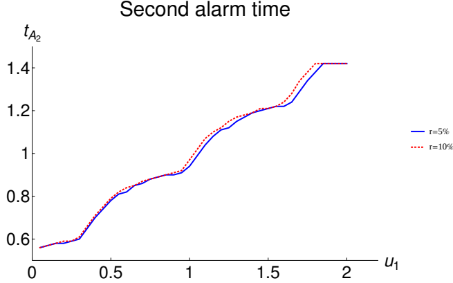
Figure 3.5: The second alarm time t_{A_2} for different values of u_1 . Parameter values: \lambda = 2 , \alpha = 0.7 , u_0 = 10 , u' = 2 , c = 1 , a = 0.4 , b = 0.25 and d = 4 . Blue (solid) and red (dotted) lines represent r = 5\% and r = 10\% respectively.
