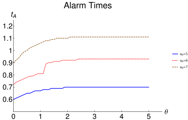
Figure 3.1: Alarm time t_A against dependence level \theta , based on Example 3.2.4. Parameter values: \lambda = 1 , \alpha = 5 , \beta = 2 , c = 10 , a = 0.4 , b = 0.1 , d = 2 and y = 0.5 . Blue (solid), red (dotted) and brown (dashed) lines represent u_0 = 5, 6, 7 respectively.
