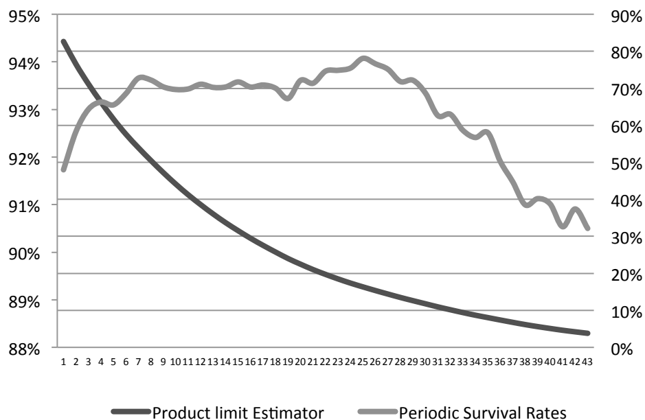
FIGURE 2-2: PRODUCT LIMIT ESTIMATOR AND CONDITIONAL SURVIVAL PROBABILITIES OF THE PLE
