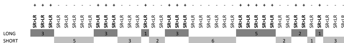
FIGURE 1-3: GRAPHICAL DESCRIPTION OF DURATION DATA
