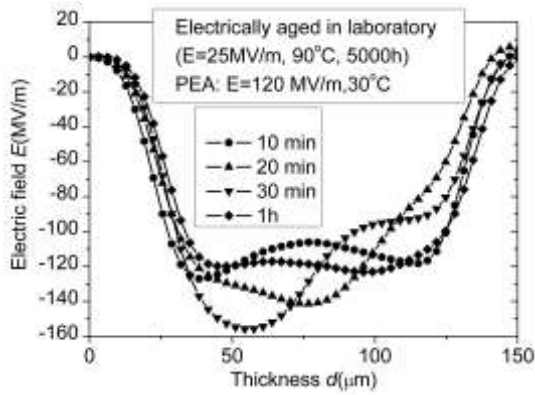
Fig. 1. Electric field distribution at selected times during transit of the sample by a charge packet at T = 30^\circ\text{C} . Taken from [11]
