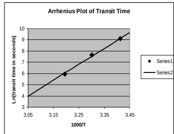
Fig.4. Arrhenius plot of transit time (diamonds) and line fitted to an activation energy of 1.22\text{ eV}
