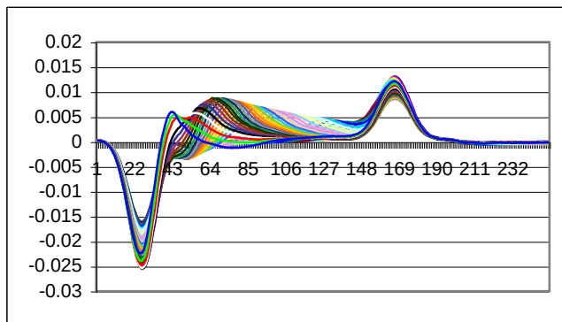
Fig.2. Charge packet transit over first 6.12 min. at T = 40^\circ\text{C} (deconvolved but uncalibrated data)
