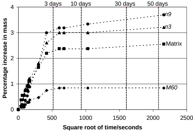
Figure 2: Water diffusion in epoxy samples (75% RH, 298K)
