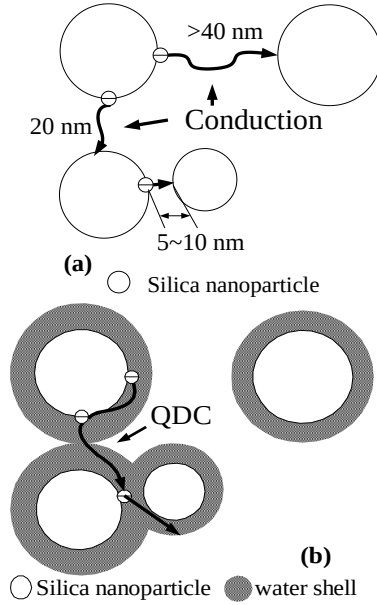
Figure 12: Charge carrier movement through overlapping water shells
