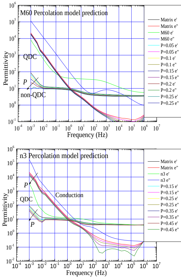
Figure 15: Calculation of complex permittivity using equation (5) for (a) micro-composite and (b) nano-composite.
