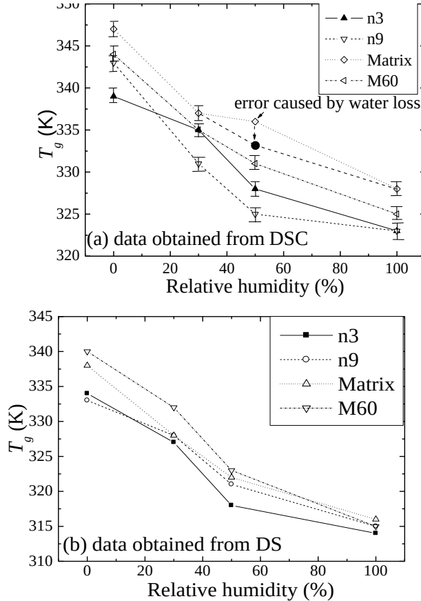
Figure 6: T_g of epoxy samples at various relative humidities. (a): measured by DSC (error ranges \pm 2 K) and (b): measured by dielectric spectroscopy (DS) (error ranges \pm 2 K)
