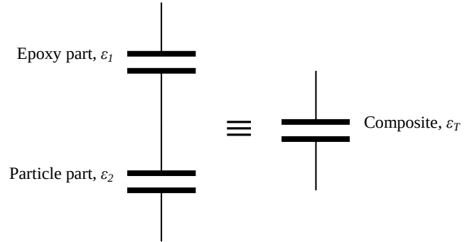
Figure 14: Consideration of particle and matrix in series
