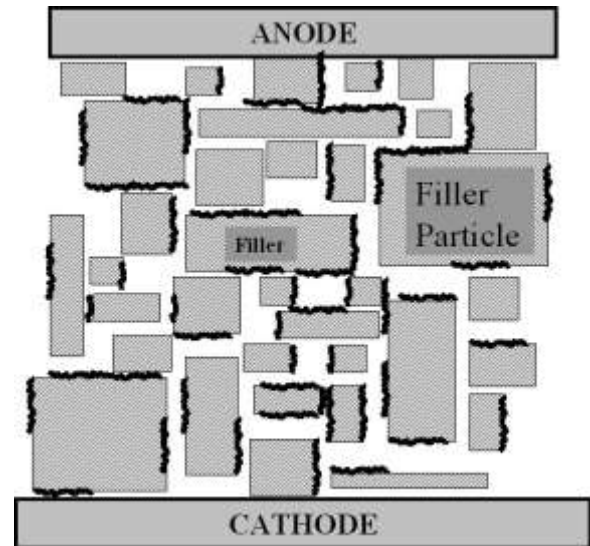
Figure 16: Interface degradation aging scenario (from [40])
