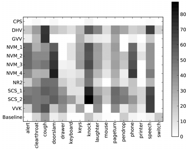
Fig. 3. Event detection (OL) results in class-wise F (%) for each event class separately.
