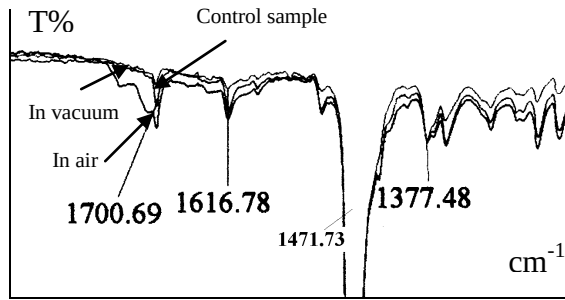
Figure 2. FTIR spectra of LDPE irradiated in different atmospheres
