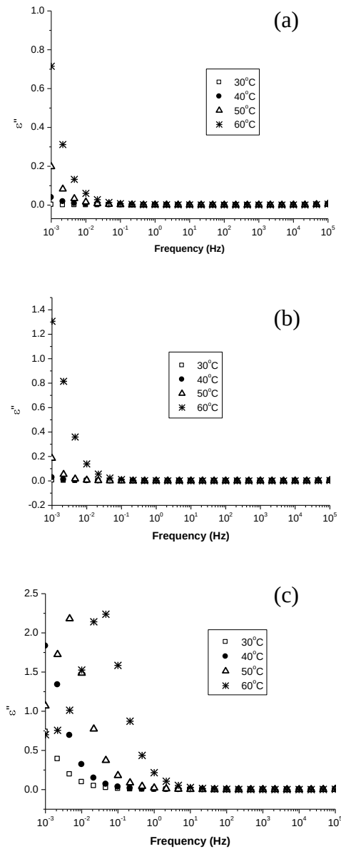
Figure 3. Spectra of dielectric loss factor of samples irradiated with 100kGy in (a) nitrogen (b) vacuum and (c) air, for a range of temperatures.
