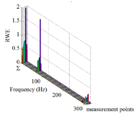
Figure 13: Scale-dependent RWE(j) in (16) and RWE in (10) (denoted by \Sigma ) using the Meyer wavelet filter bank of Table 2 for the space truss of Figure 6 subject to (a) the sine-sweep and (b) the white noise excitation in Figure 8.
