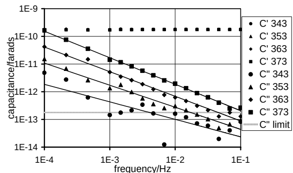
Figure 1: Low Frequency Dielectric Spectroscopy on XLPE cable samples. ‘C’ limit’ is the noise floor of the instrument.
