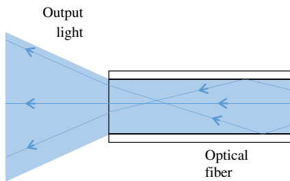
Fig. 1 Diagram of light leaving the tip standard multimode optical fiber. It disperses out in a cone dependent on the angles of light rays within the core. The angle of divergence of the cone gives the numerical aperture.
