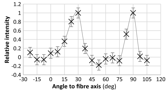
Fig. 11 Graph of the variation of output intensity with angle for the angle-tipped optical fiber. There is a peak diffracted out from the tip of the fiber, shifted to around 30 deg, and a second peak reflected from the tip centered around 90 deg. Errors come from the limit of sensitivity of the power meter. The resolution of these relative intensity measurements was 0.15.
