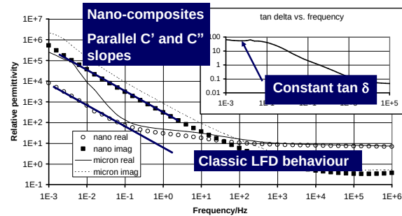
Figure 11: Dielectric spectrum: epoxy – \text{TiO}_2 NANO-composite [39]
