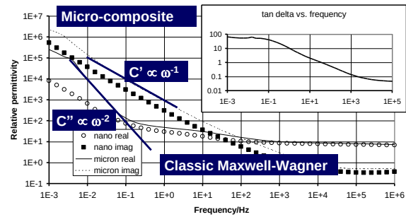
Figure 10: Dielectric spectrum: epoxy – \text{TiO}_2 MICRO-composite [39]
